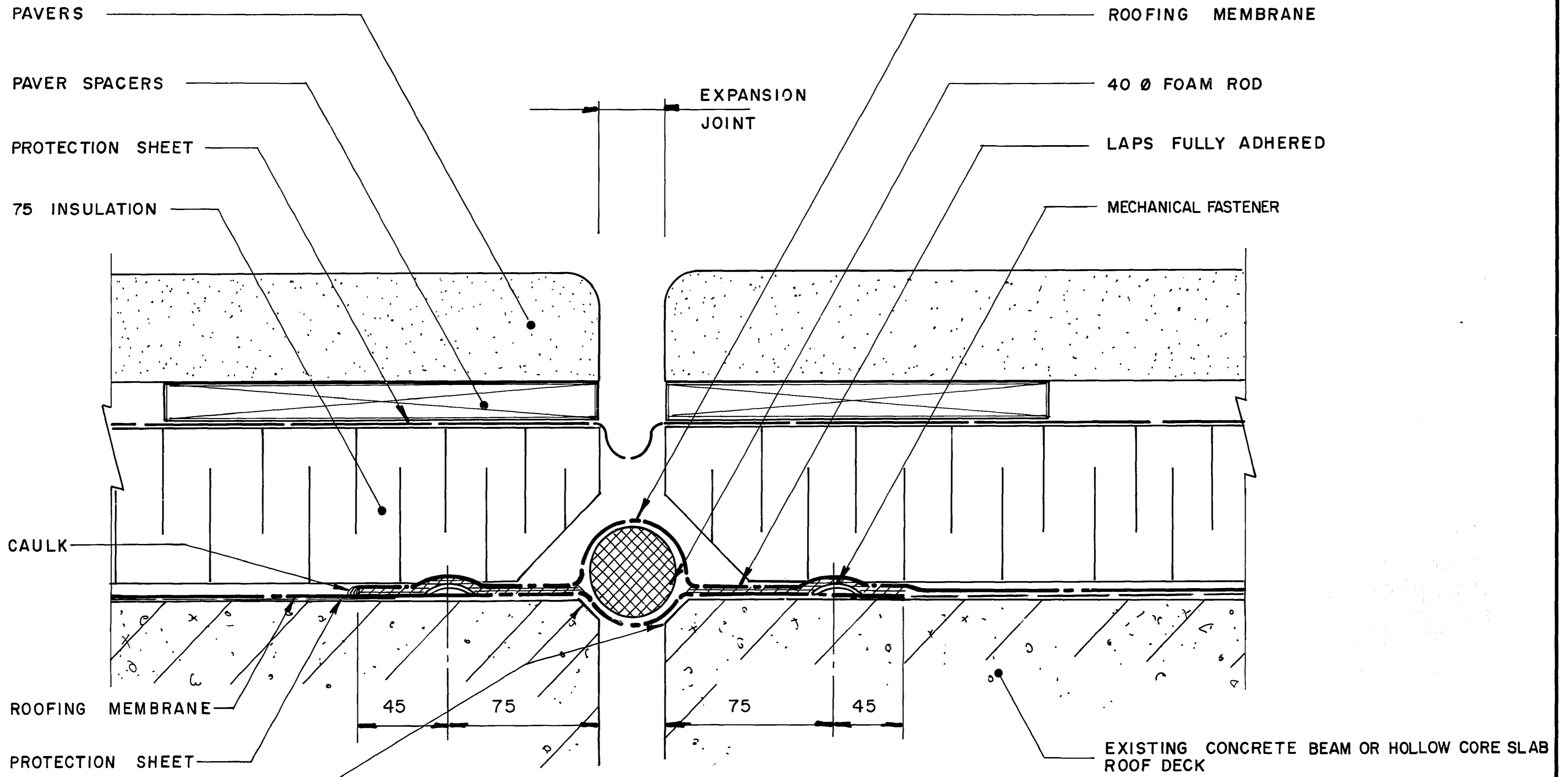
1 TYPICAL EXPANSION JOINT SD-03 1:2
