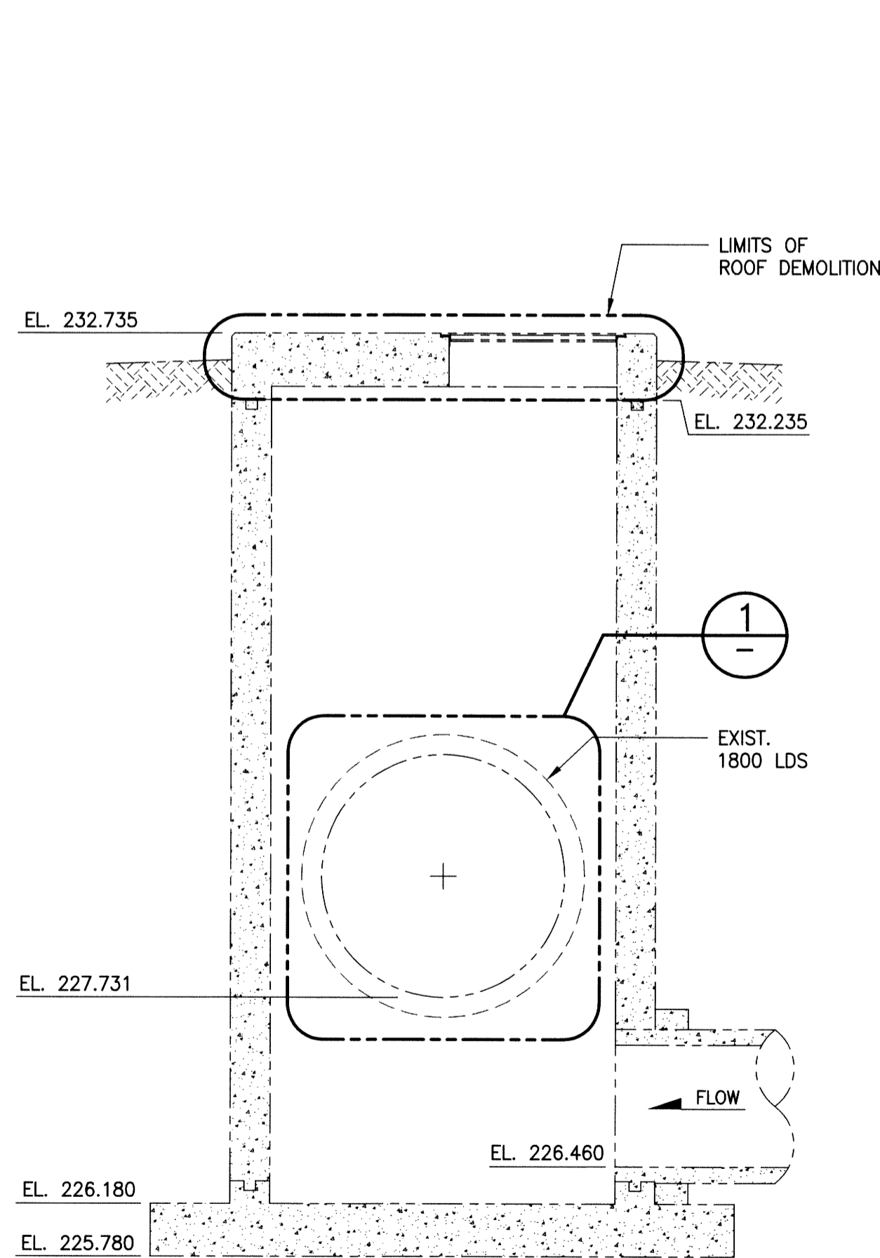
SECTION (LOOKING SOUTH) SCALE: 1:40
