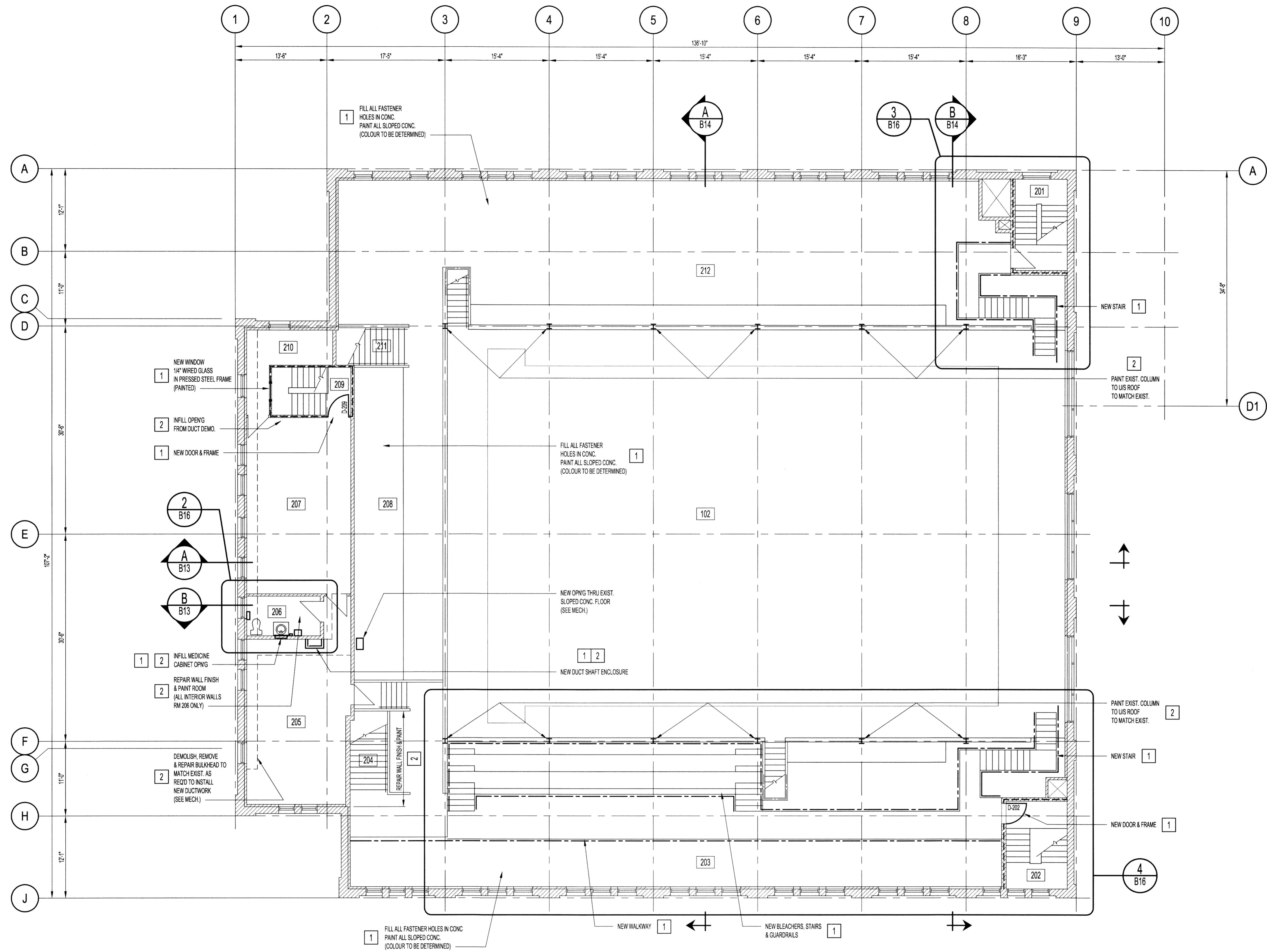
MEZZANINE PLAN - RENOVATED SCALE: 1/8"=1'-0"
