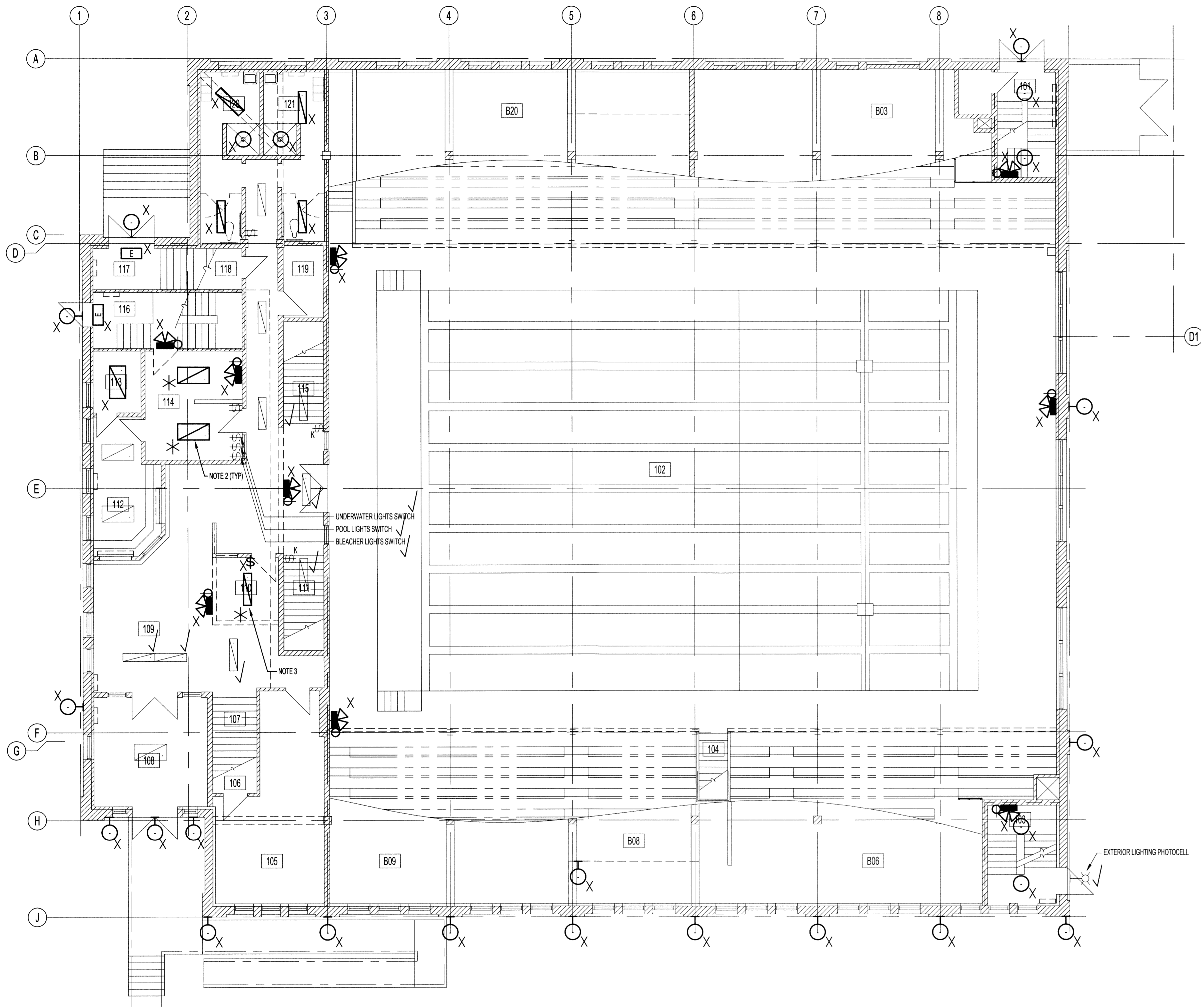
MAIN FLOOR PLAN - LIGHTING DEMOLITION SCALE: 1/8"=1'-0"
