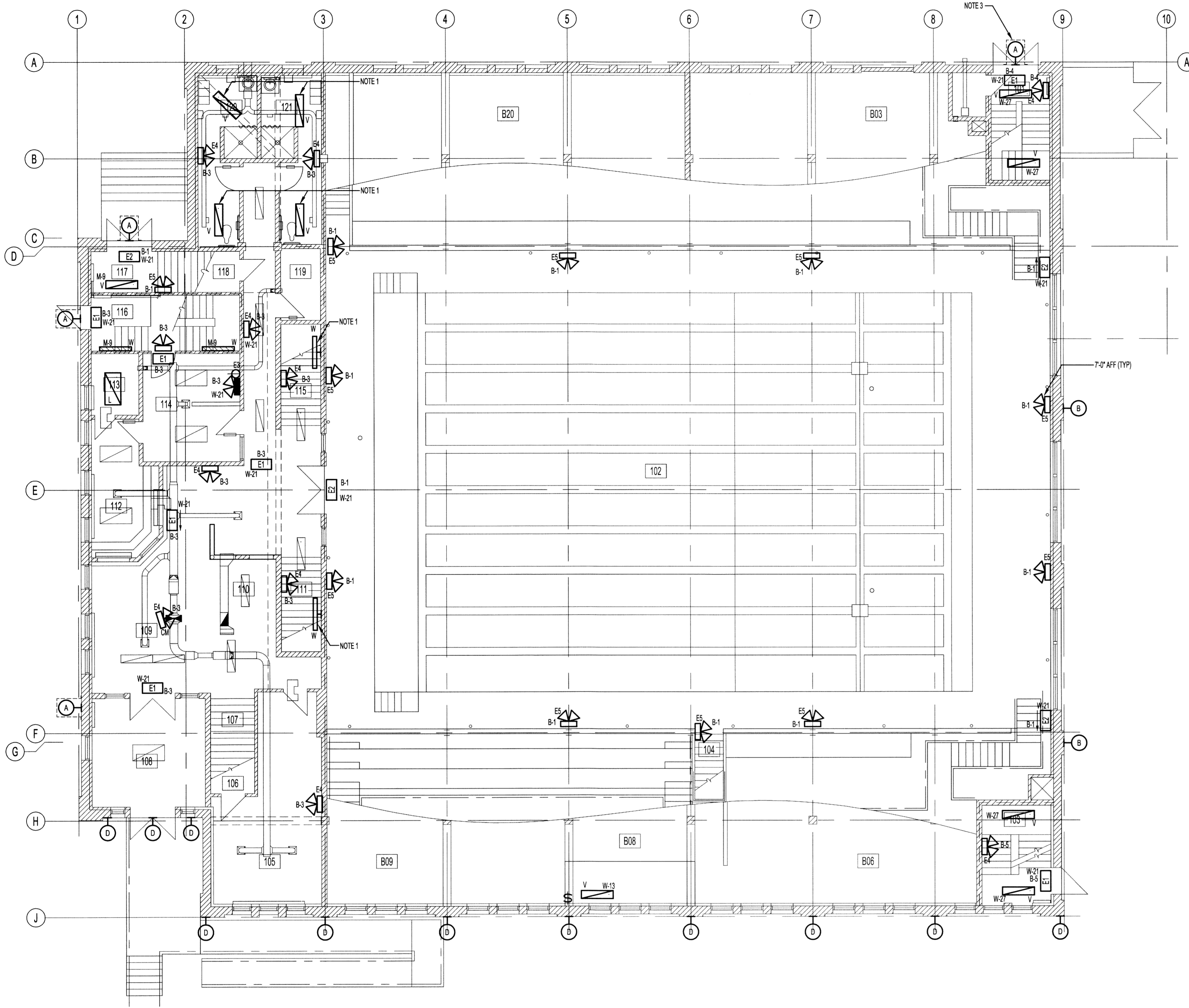
MAIN FLOOR PLAN - LIGHTING SCALE: 1/8"=1'-0"
