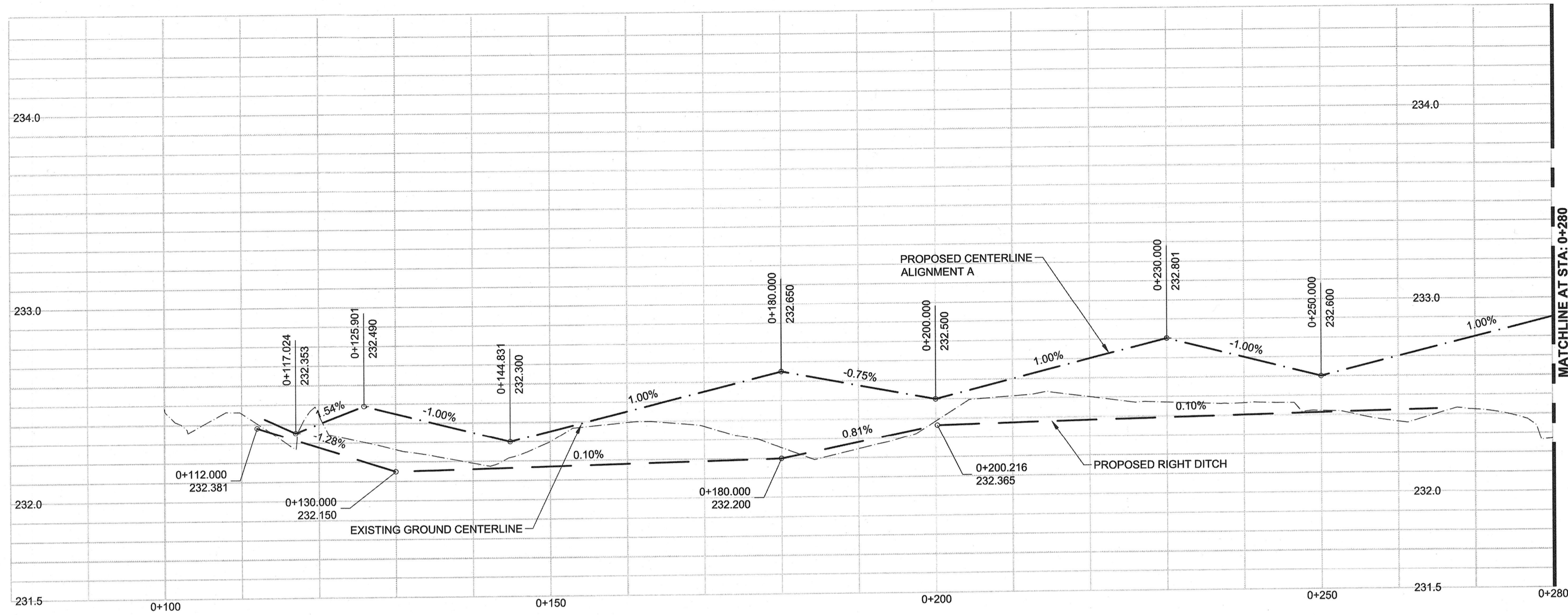
ALIGNMENT A - PERIMETER ROAD PROFILE - WEST LEG
