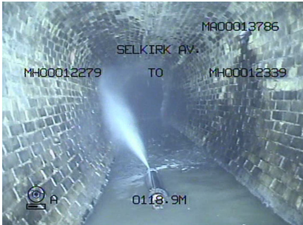
Figure 16 – Selkirk Ave Trunk, 118.9m downstream of MH00012279, facing east
