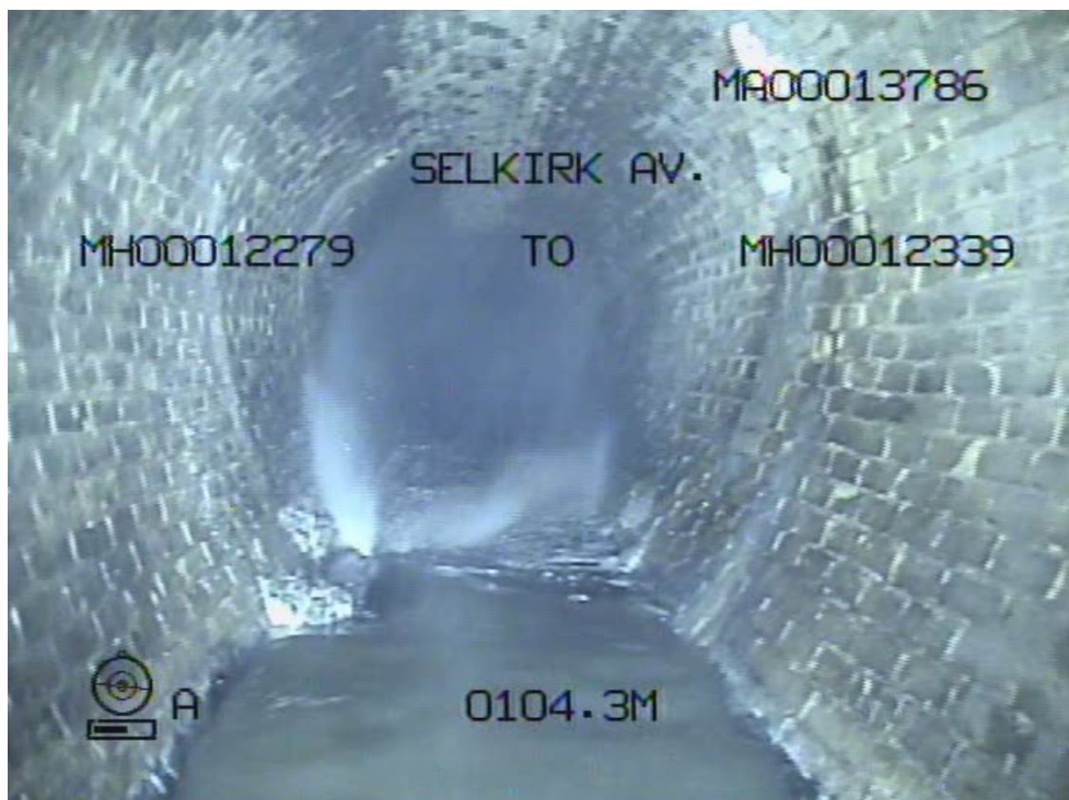
Figure 15 – Selkirk Ave Trunk, 104.3m downstream of MH00012279, facing east
