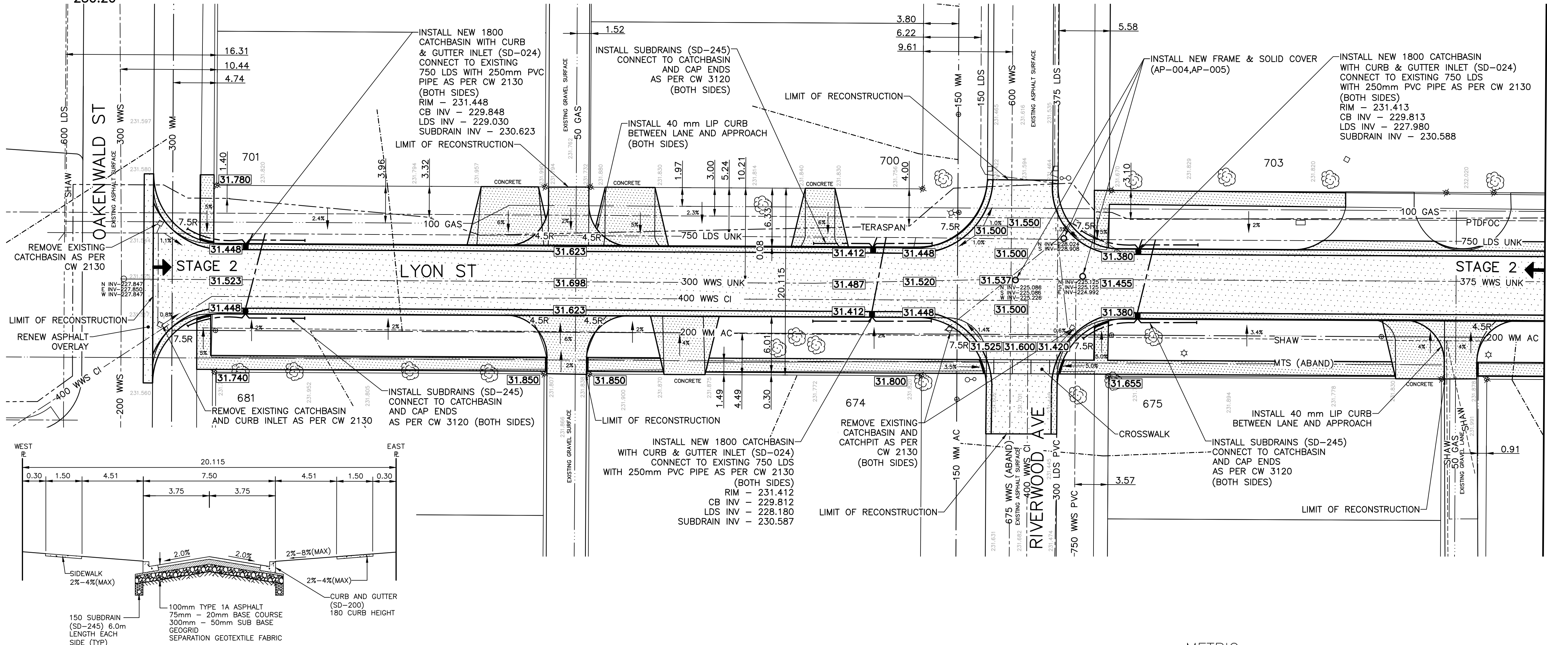
TYPICAL CROSS SECTION N.T.S.
