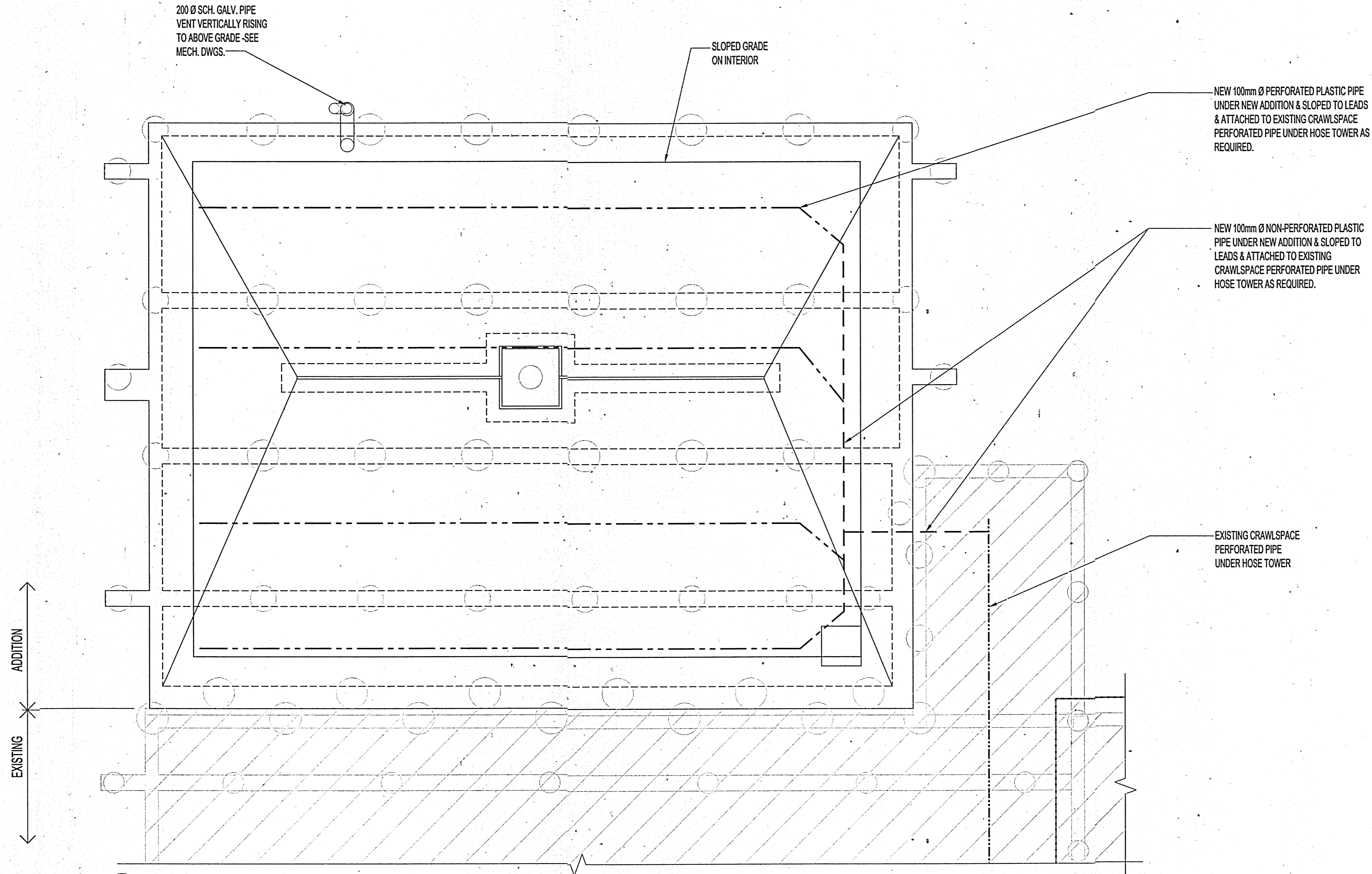
2 PARTIAL MAIN FLOOR CRAWLSPACE PLAN A3 SCALE 1:50
