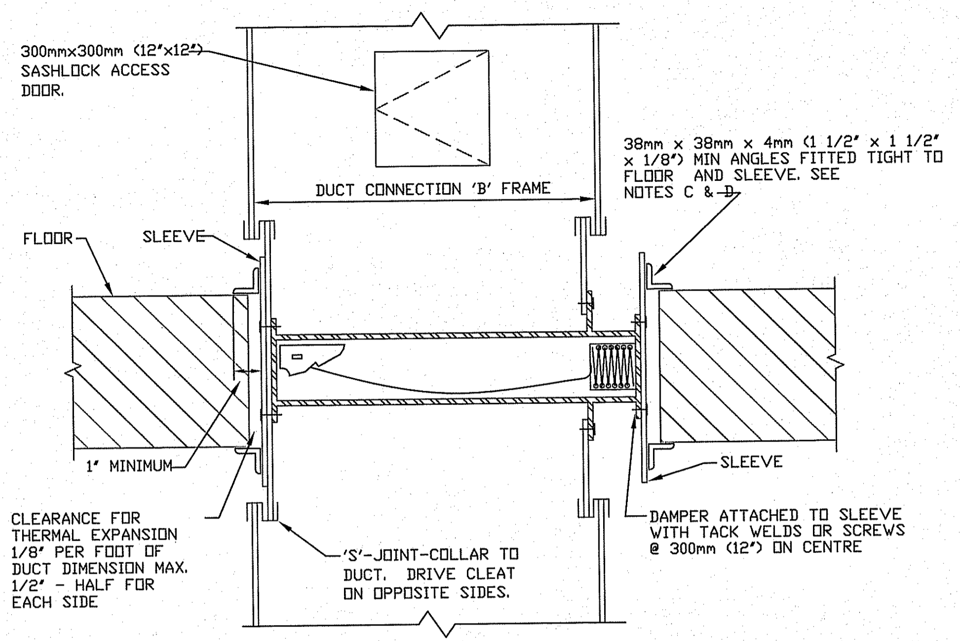
2 VERTICAL FIRE DAMPER DETAIL SCALE: NTS
