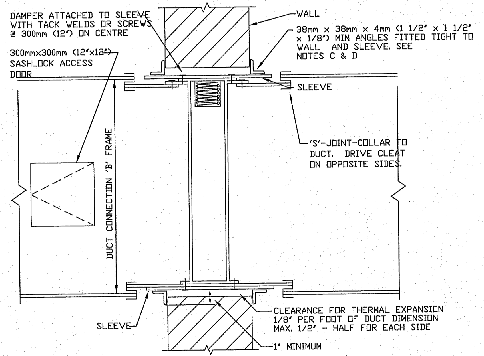
3 HORIZONTAL FIRE DAMPER DETAIL SCALE: NTS
