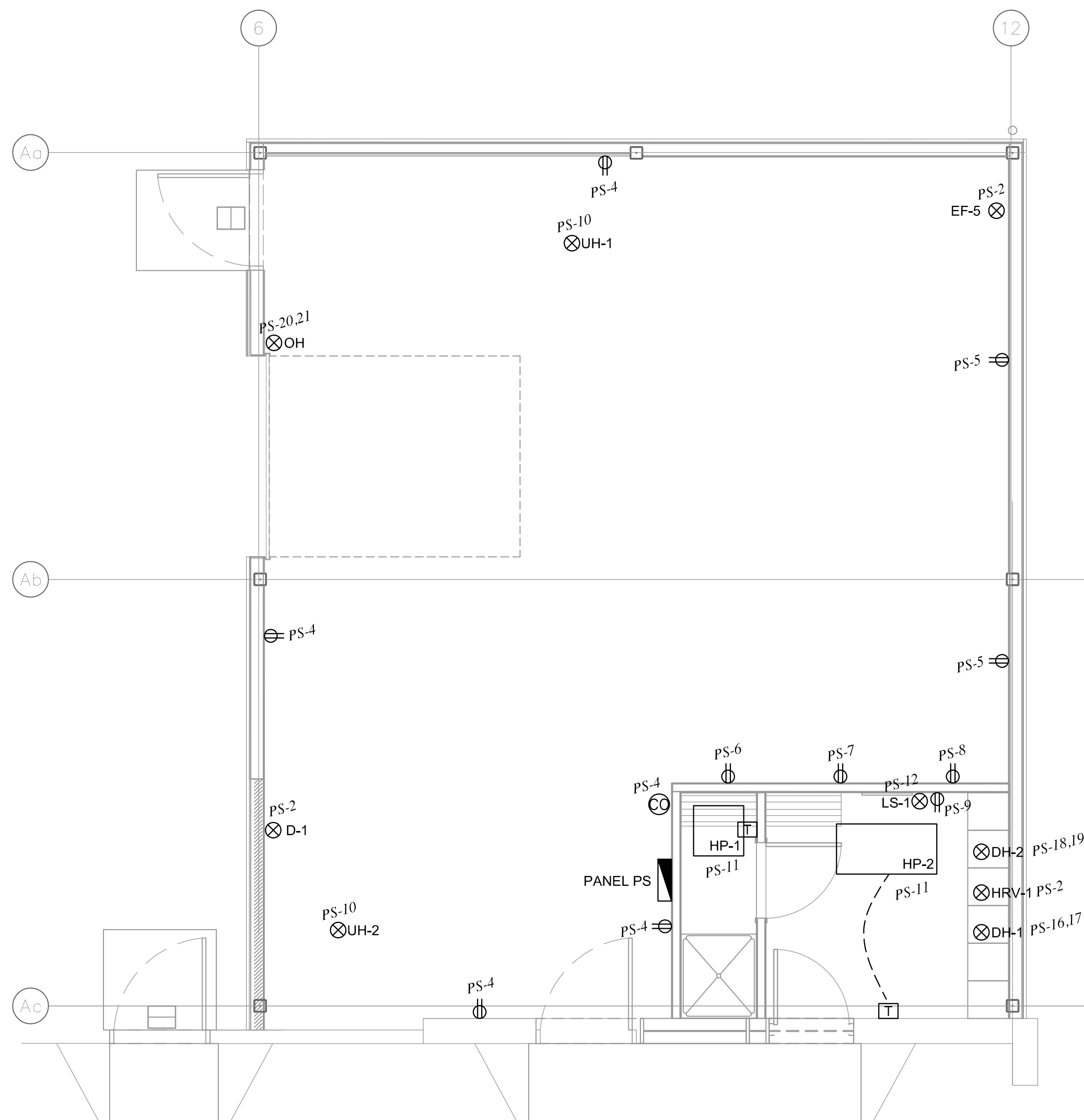
2 STORAGE ADDITION POWER PLAN E-5 SCALE: 1/4" = 1' - 0"
