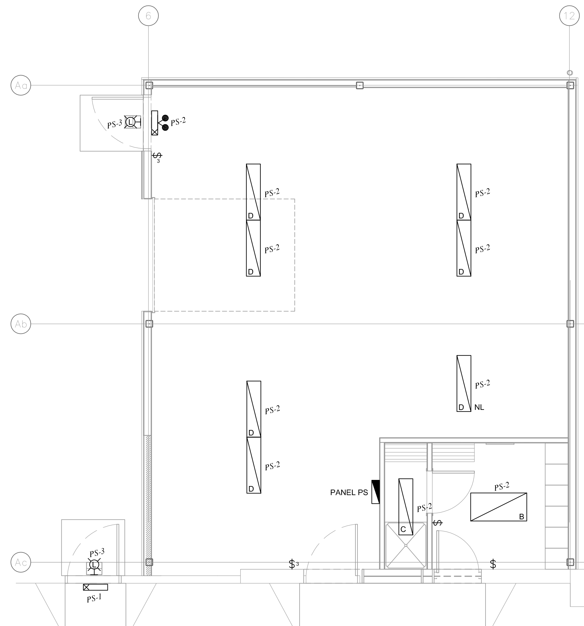
1 STORAGE ADDITION LIGHTING PLAN E-5 SCALE: 1/4" = 1' - 0"
