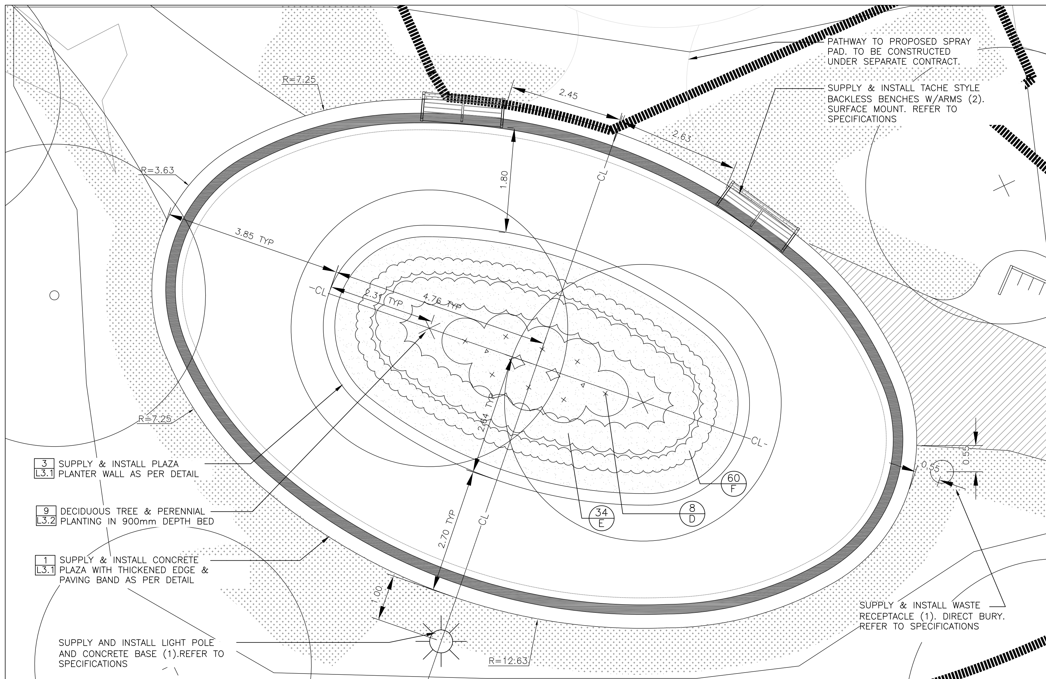
PLAZA LAYOUT & PERENNIAL PLANTING SCALE 1:50
