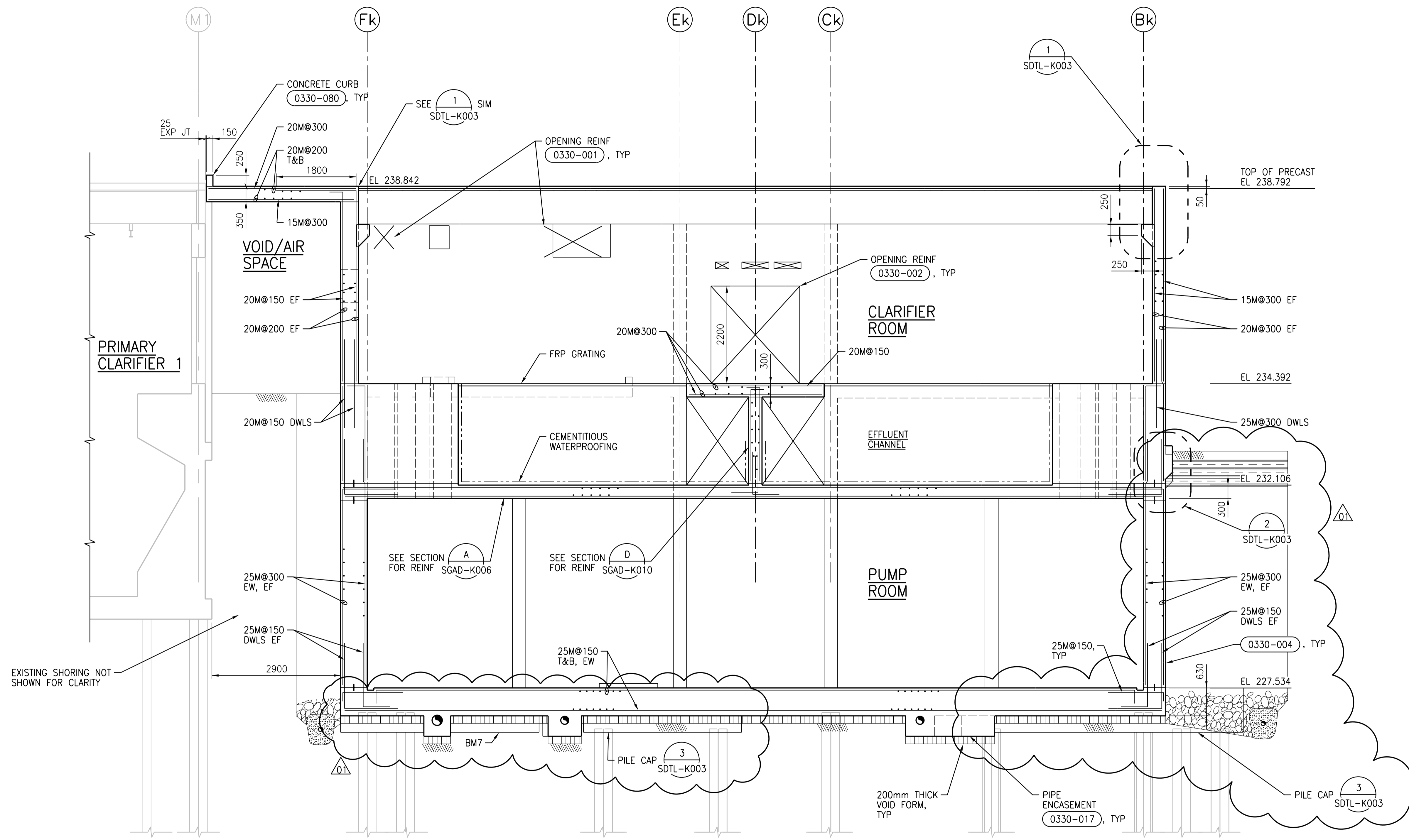
E SECTION 1:50 SCAD-K001, SCAD-K002, SCAD-K003, SCAD-K004
