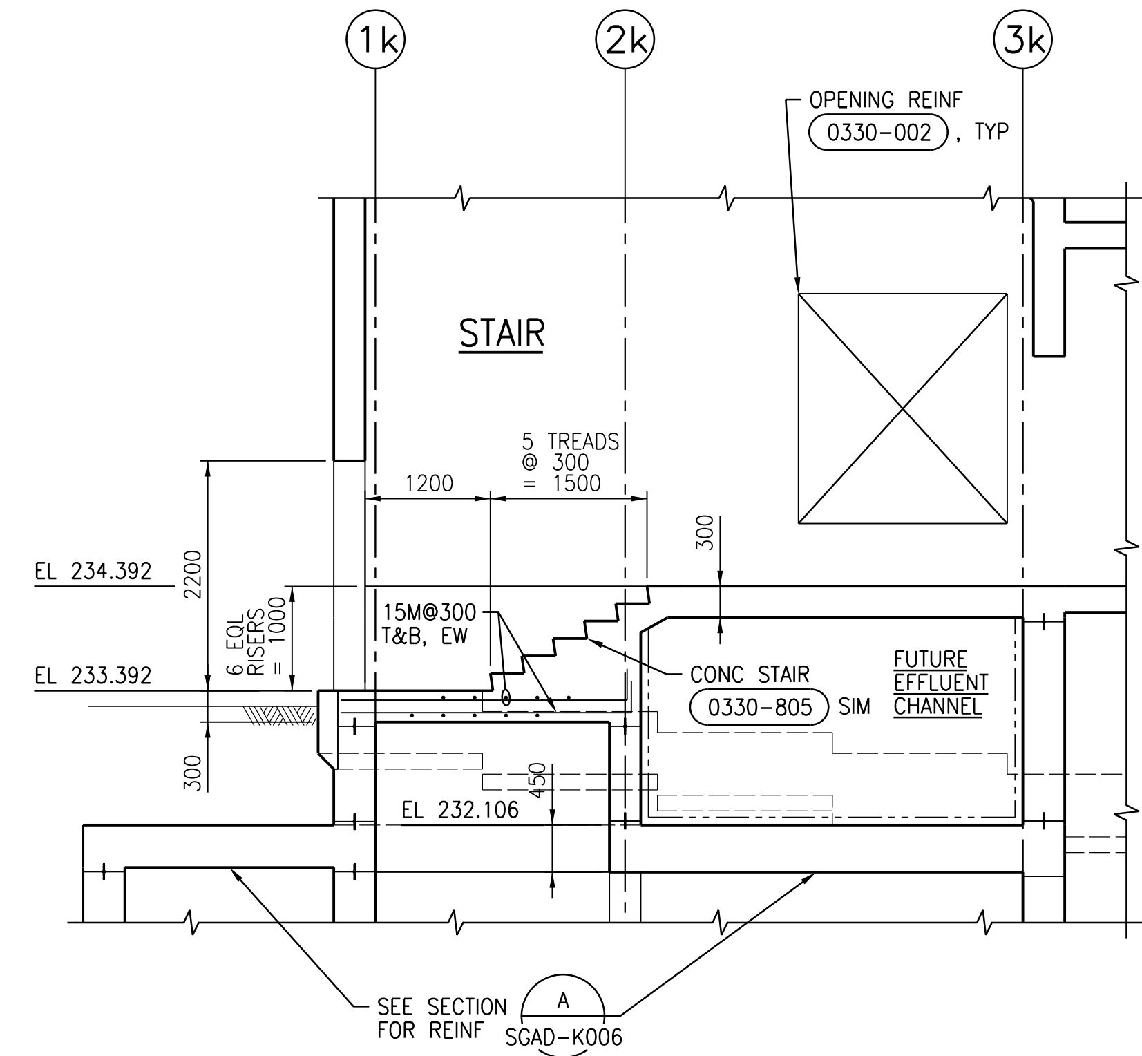
Q SECTION 1:50 SGAD-K002, SGAD-K003,
