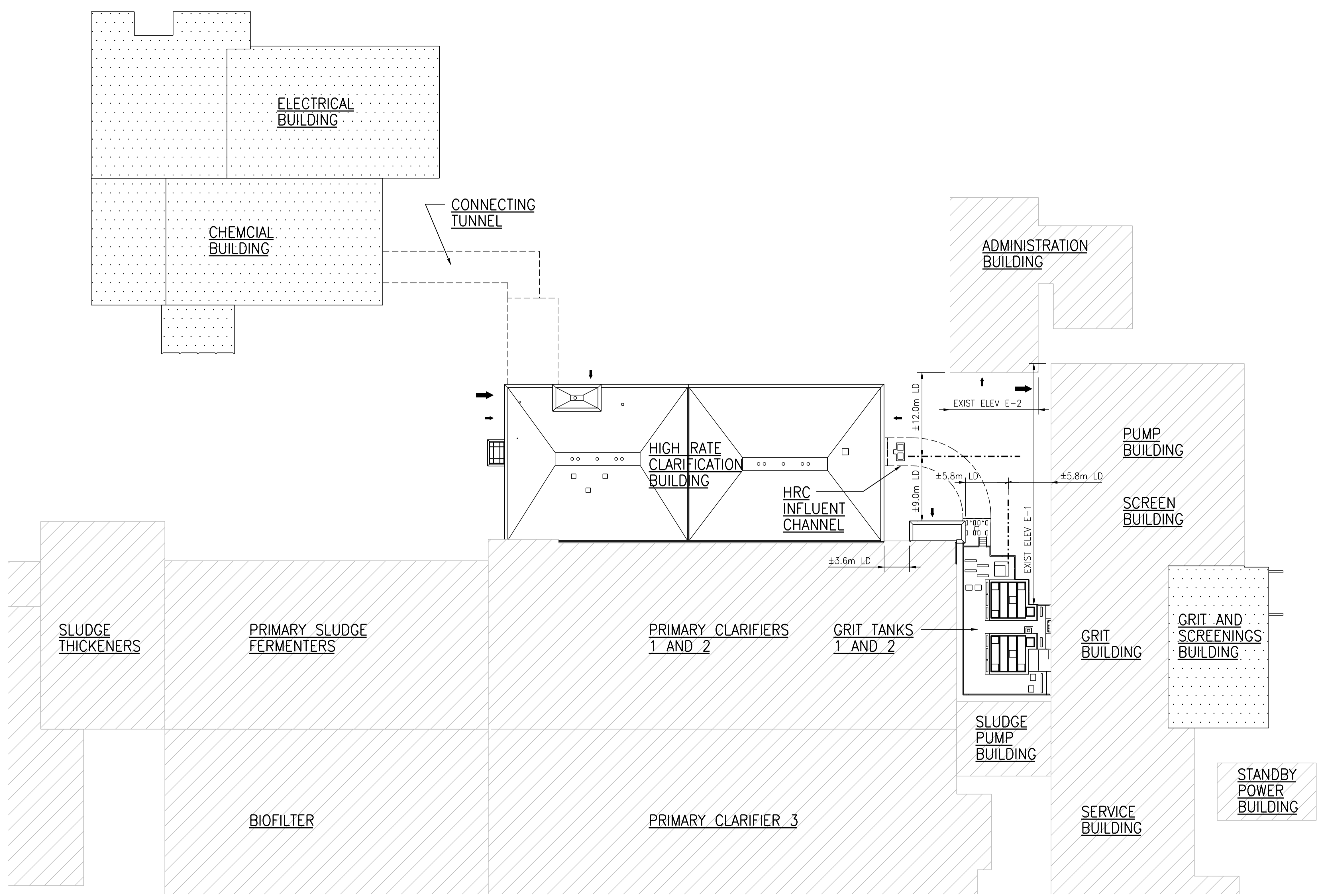
OVERALL SITE PLAN 1:300
