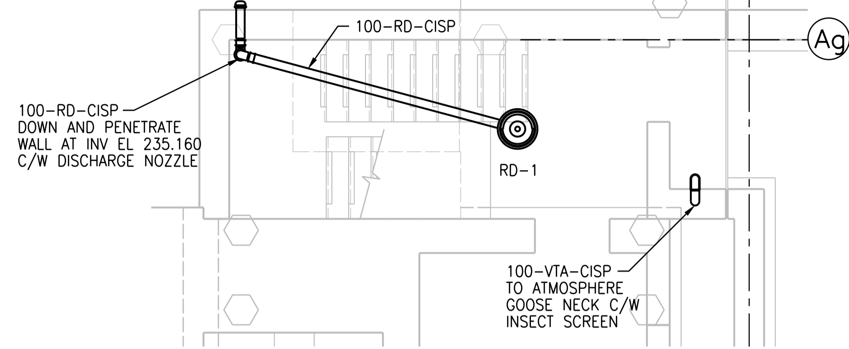
ROOF PLAN 1:50
