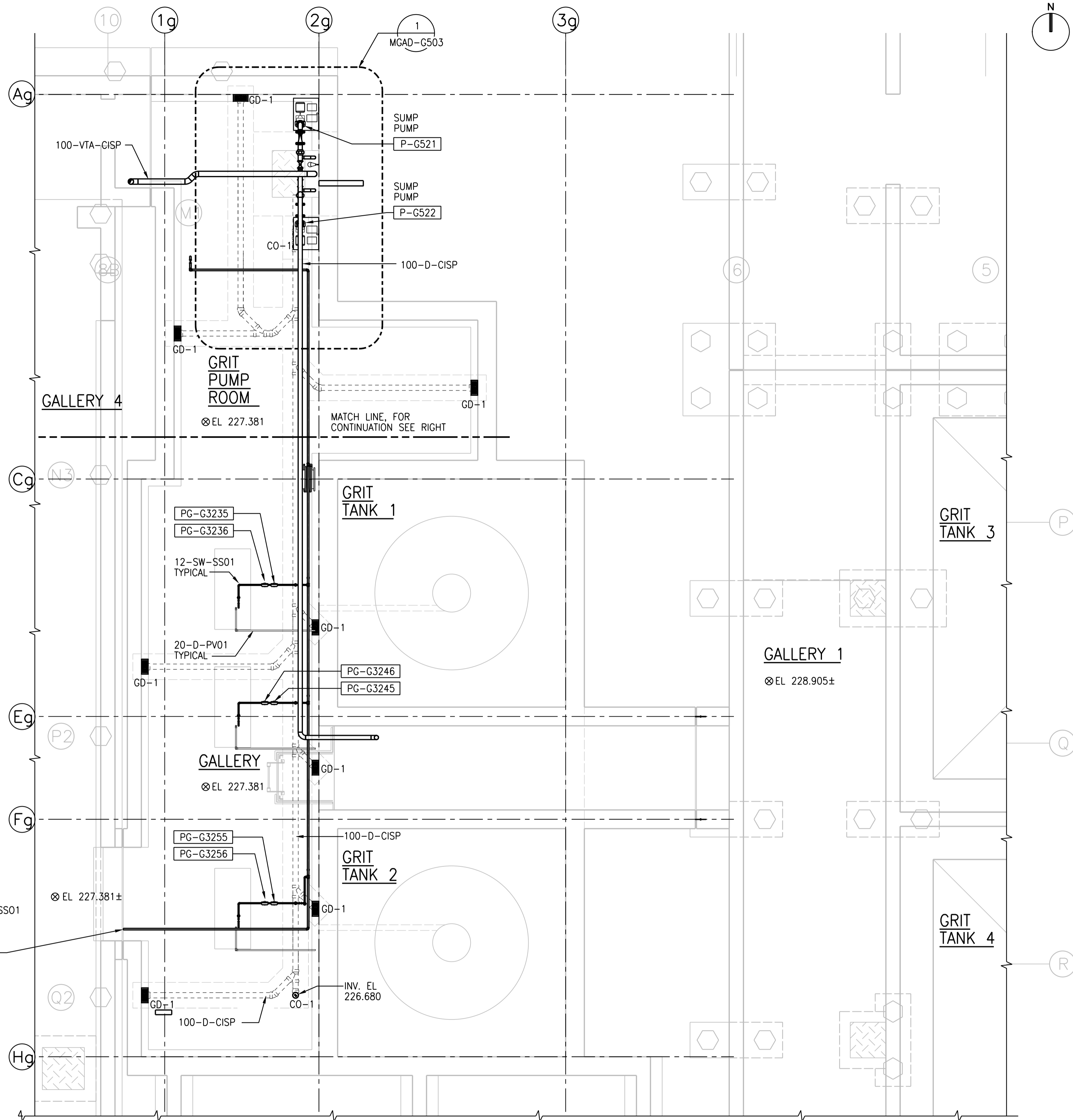
BASEMENT PLAN 1:50
