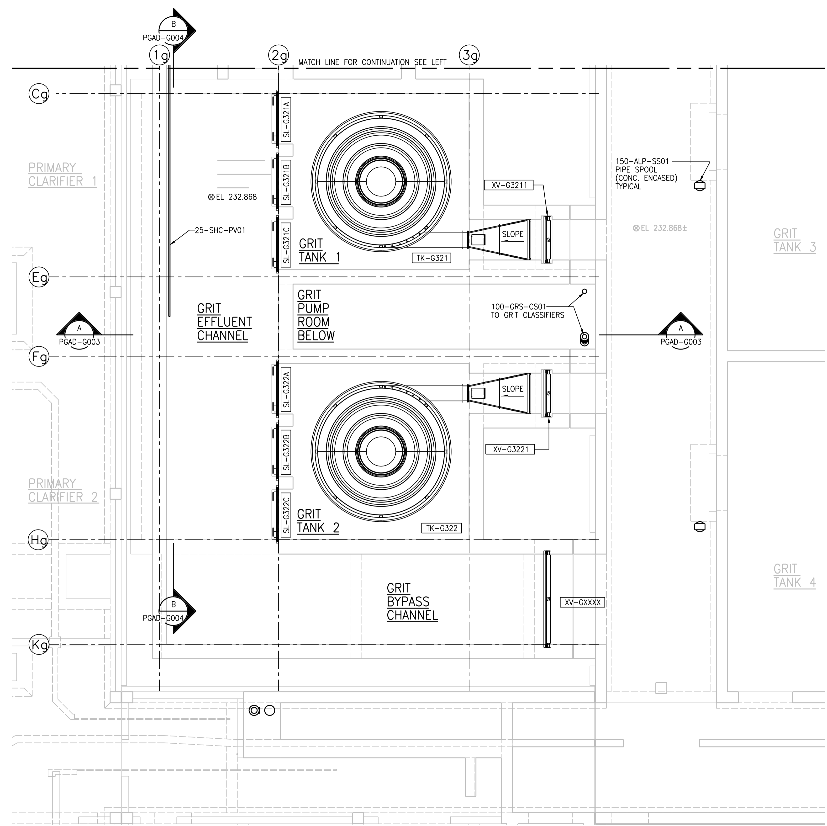
CHANNEL LEVEL PART PLAN 1:50
