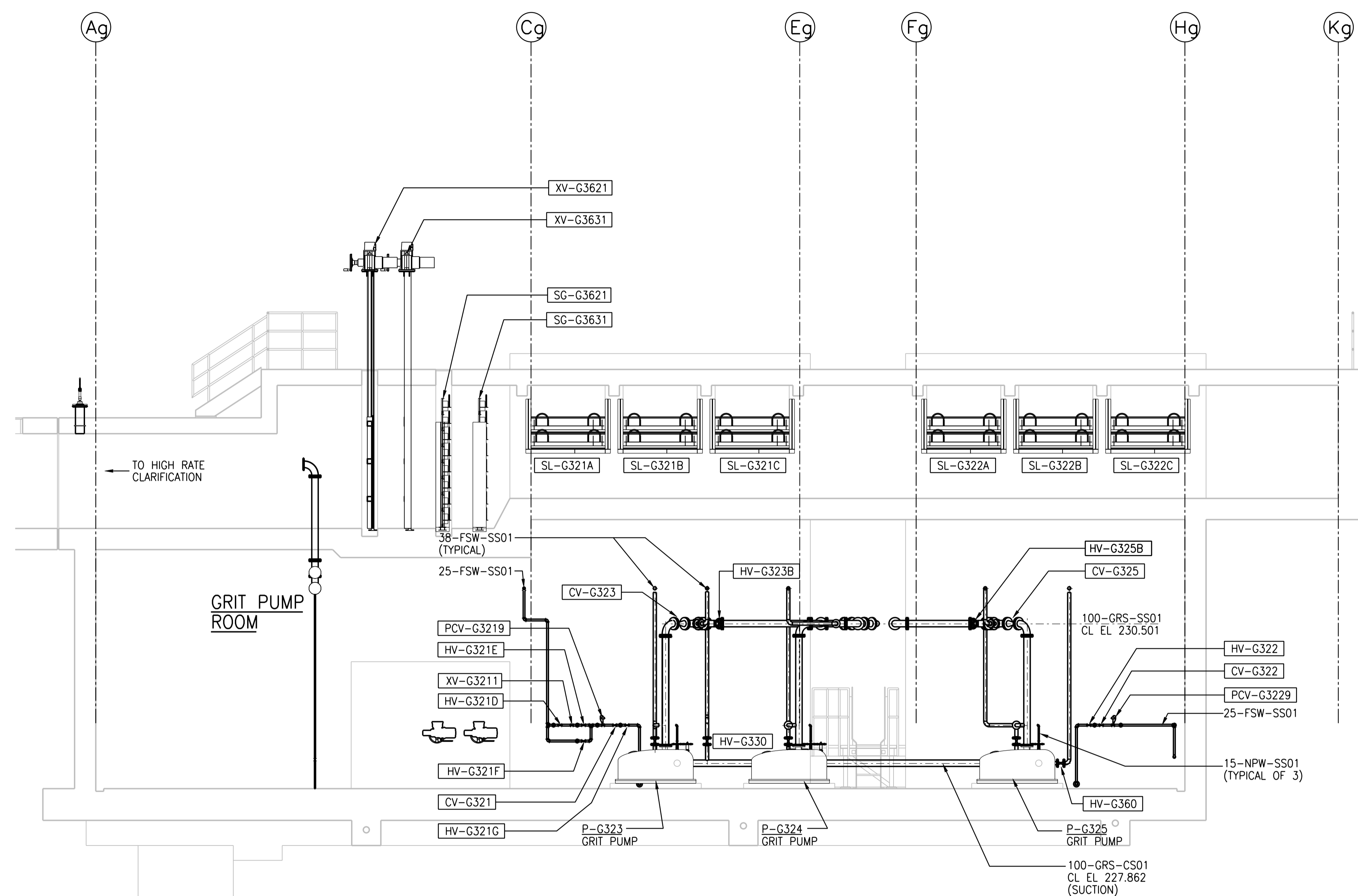
B SECTION 1:50 PGAD-G001 PGAD-G002
