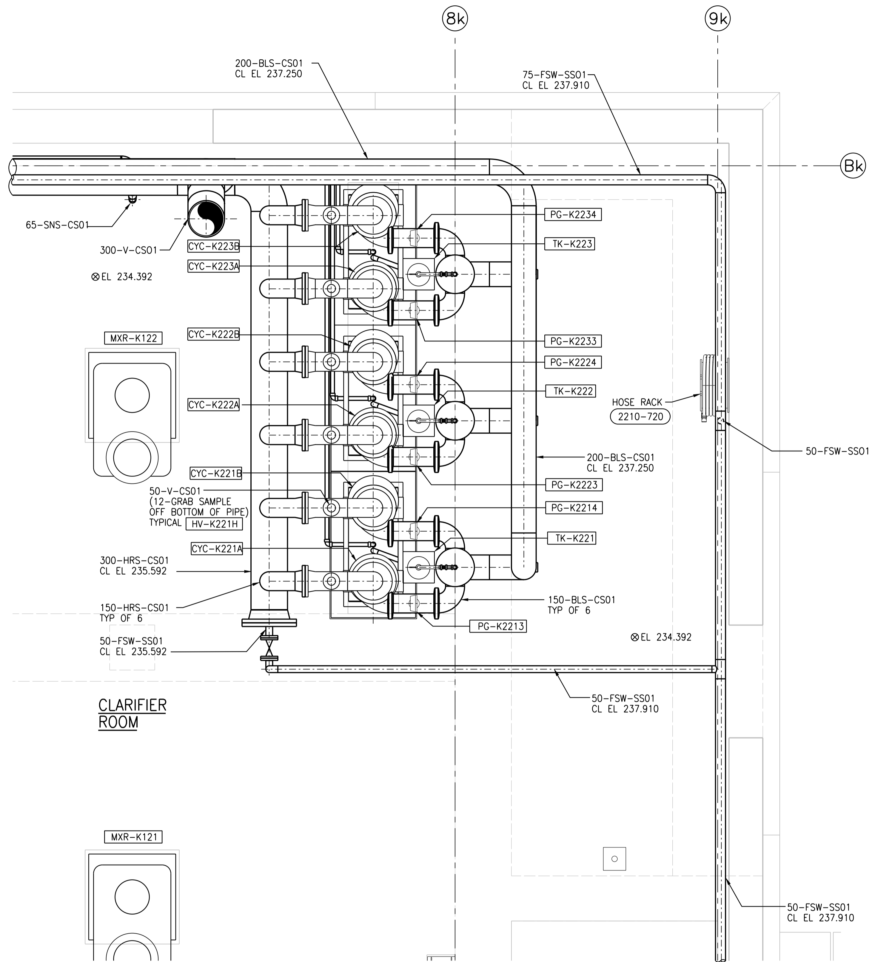
A GROUND FLOOR PART PLAN 1:20 PGAD-K002
