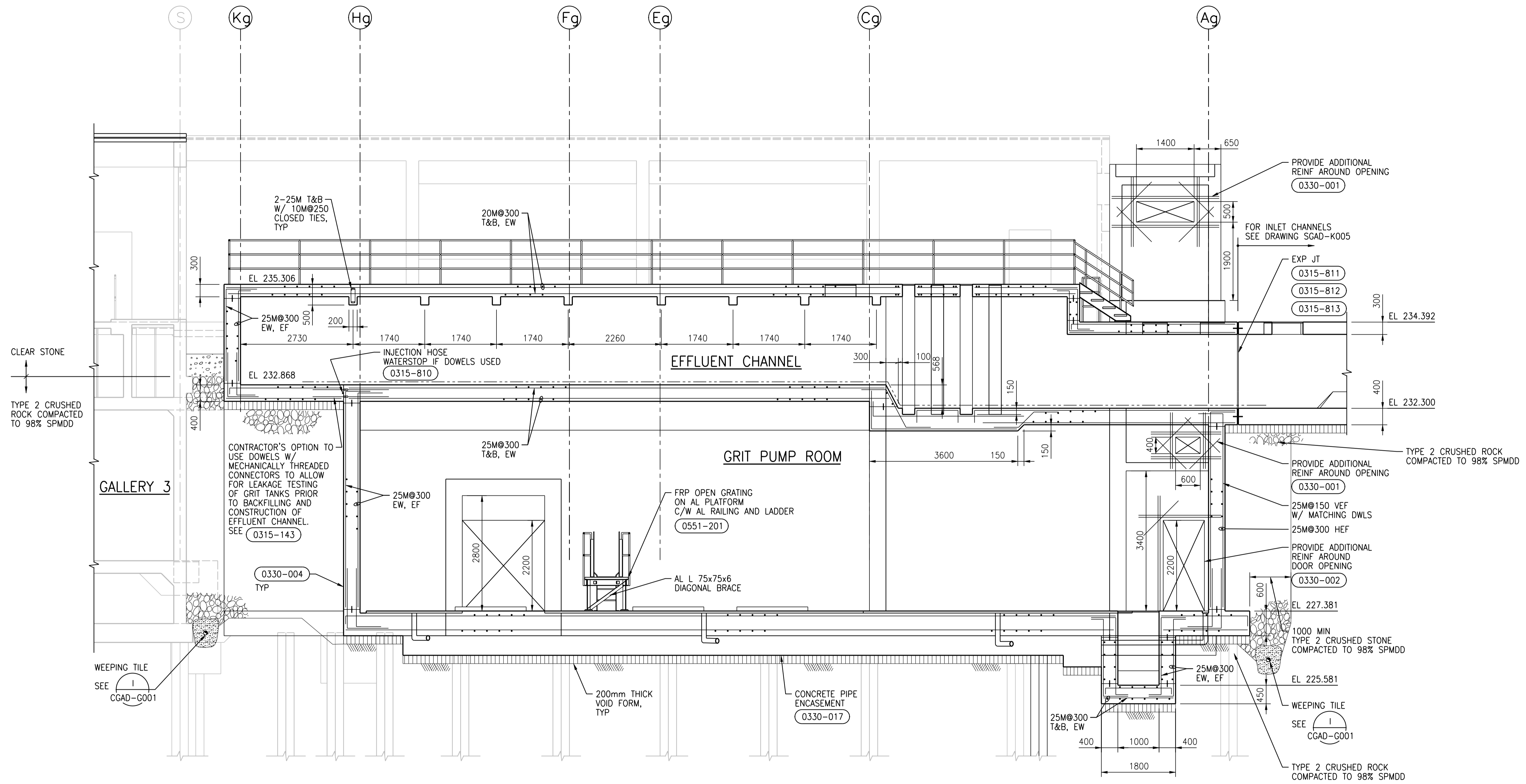
C SECTION 1:50 SGAD-G001, SGAD-G002, SGAD-G003
