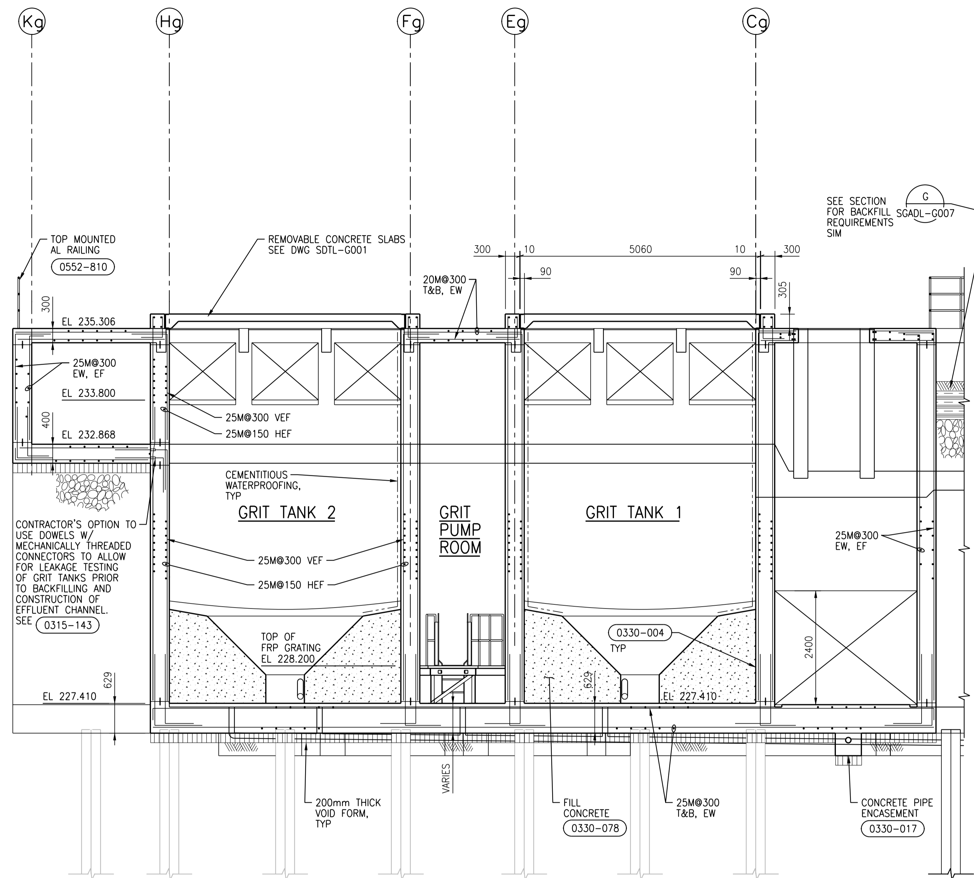
D SECTION 1:50 SGAD-G001, SGAD-G002, SGAD-G003
