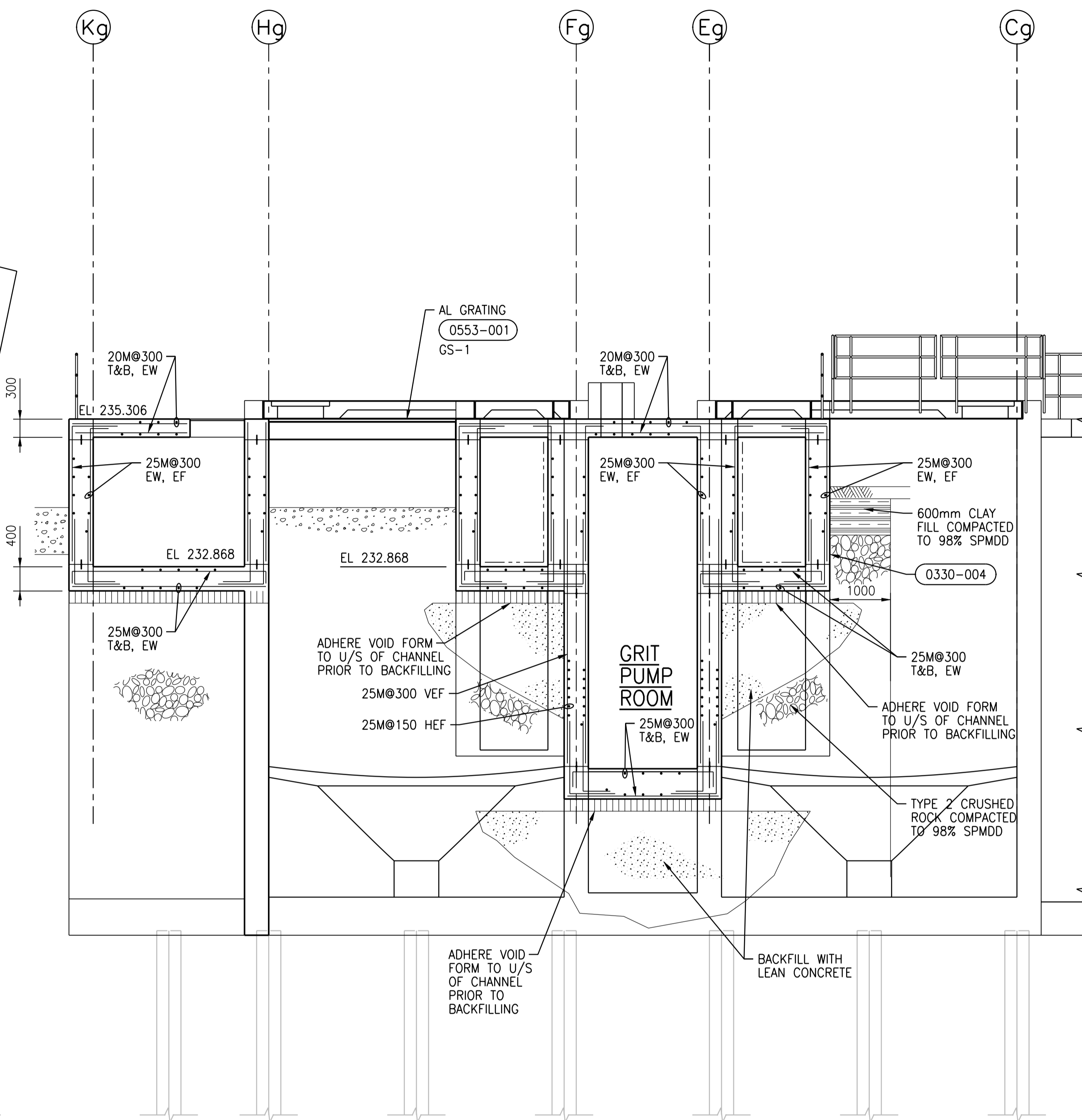
E SECTION 1:50 SGAD-G001, SGAD-G002, SGAD-G003
