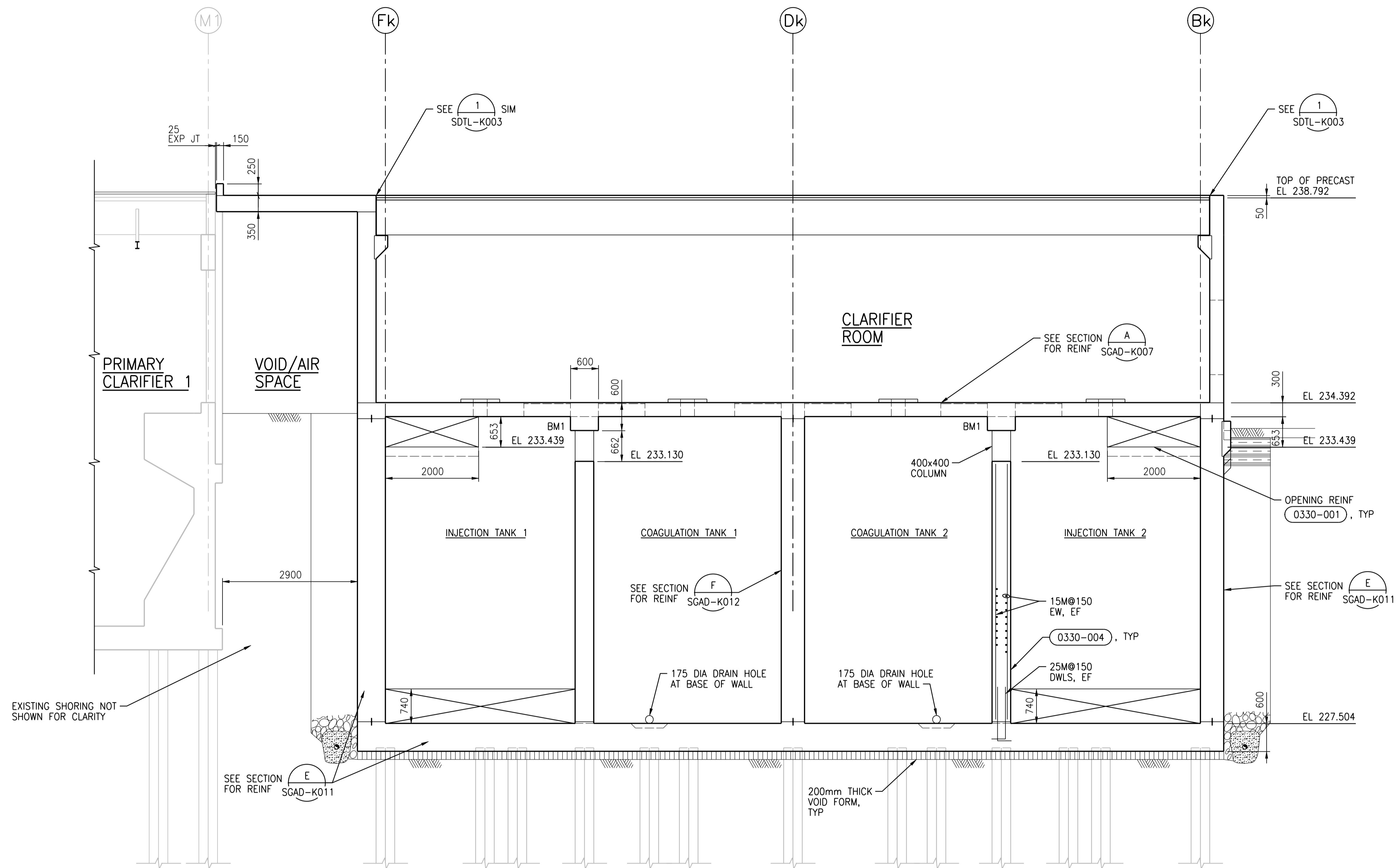
G SECTION 1:50 SGAD-K001, SGAD-K002, SGAD-K003, SGAD-K004
