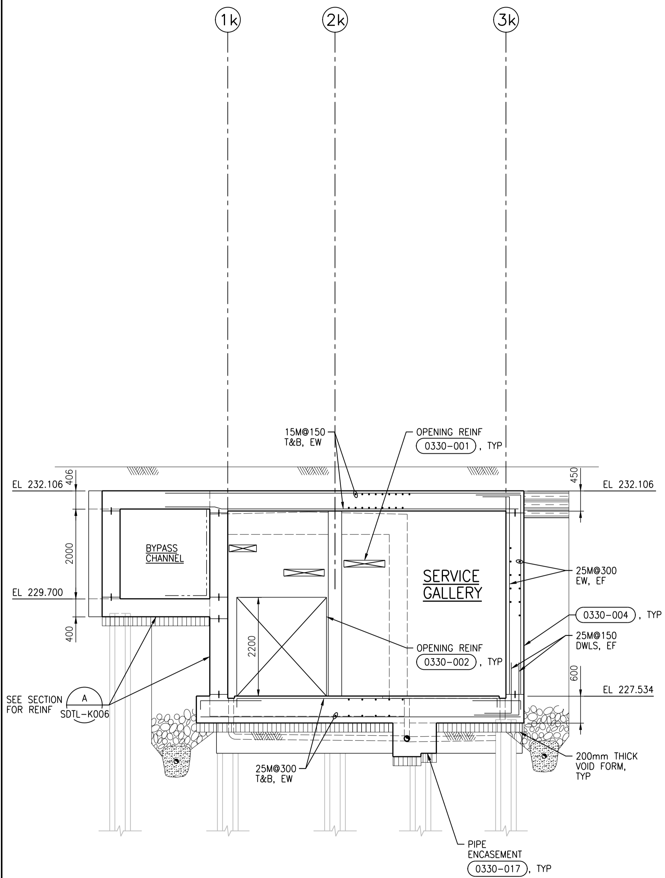
K SECTION 1:50
