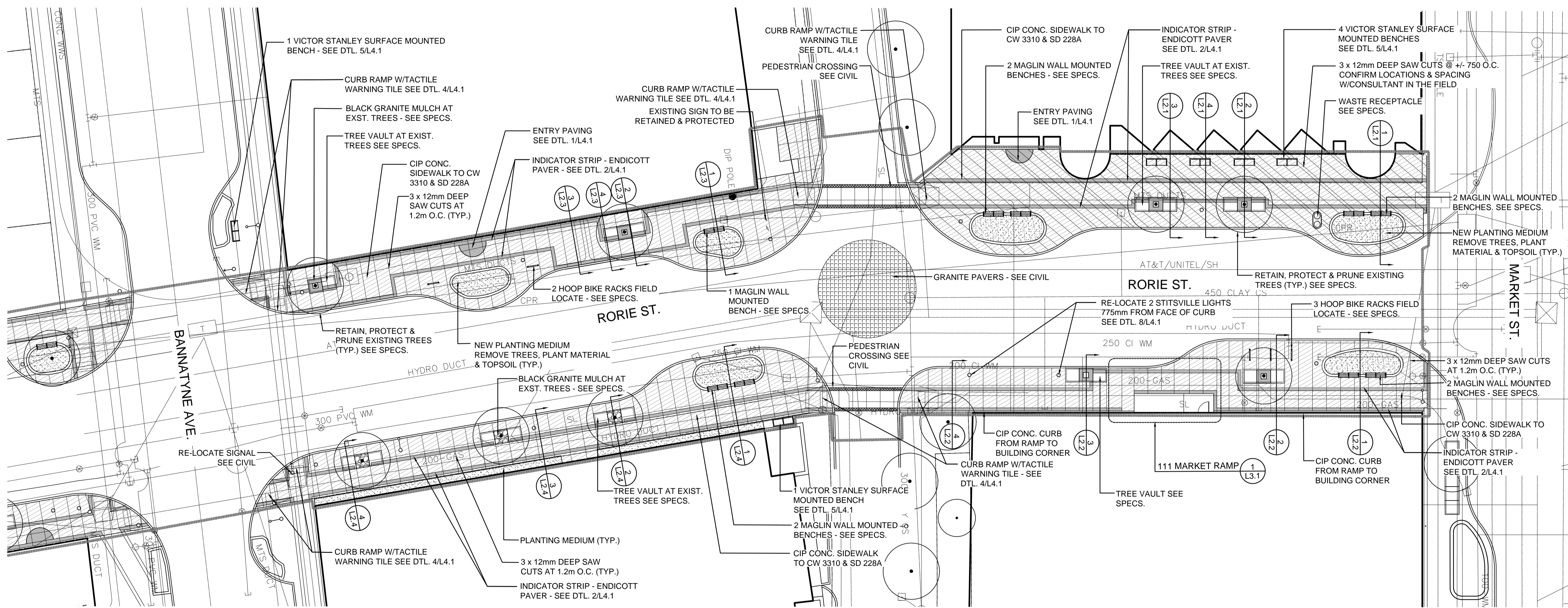
1 RORIE FROM MARKET TO BANNATYNE - MATERIALS PLAN L1.1 SCALE: 1:200
