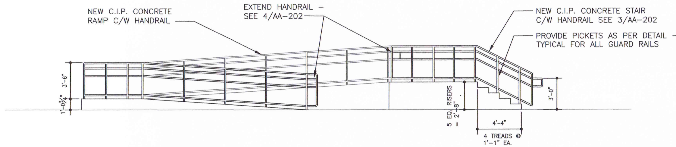
1 AA-201 (3) 3/16"=1'-0" ELEVATION DOOR 3
