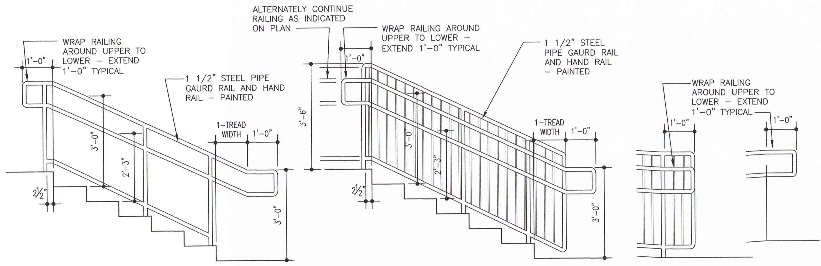
1 CENTRE RAIL DETAIL AA-202 (3) 1/2"=1'-0"
