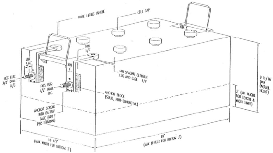
BUS BATTERY WITH DROP TERMINALS – Dimensional Specifications –
