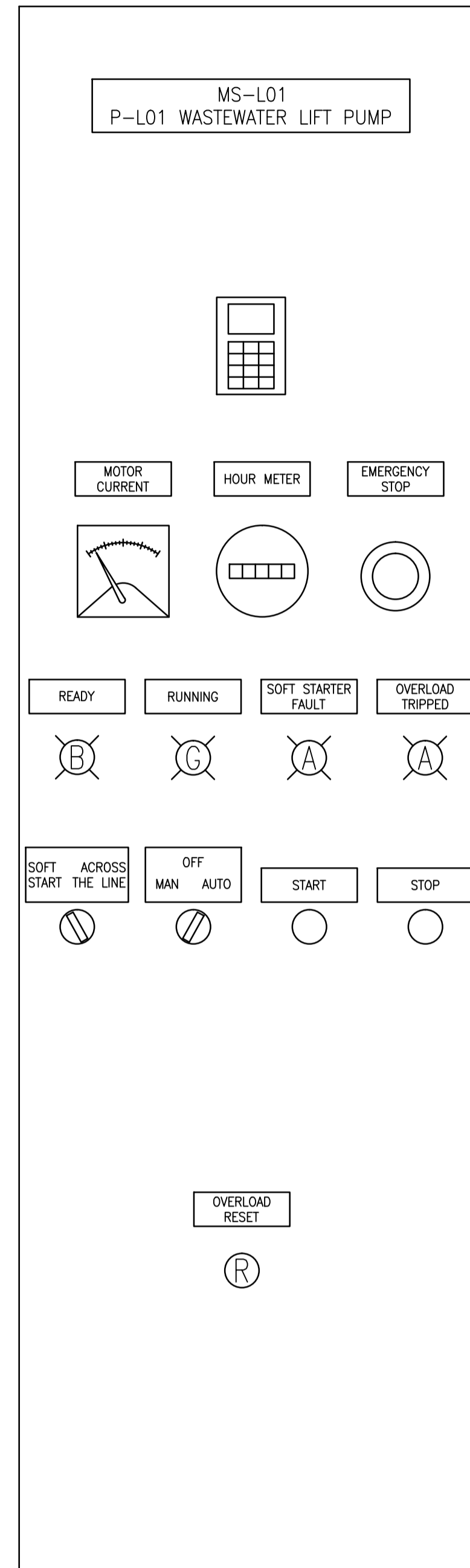
DETAIL: WASTEWATER LIFT PUMP STARTER DOOR SCALE: 1:4
