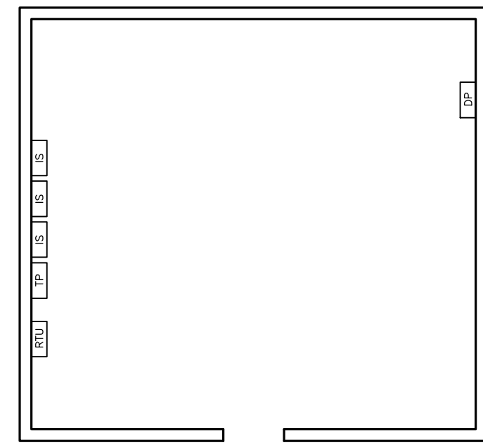
ELECTRICAL ROOM FLOOR PLAN
