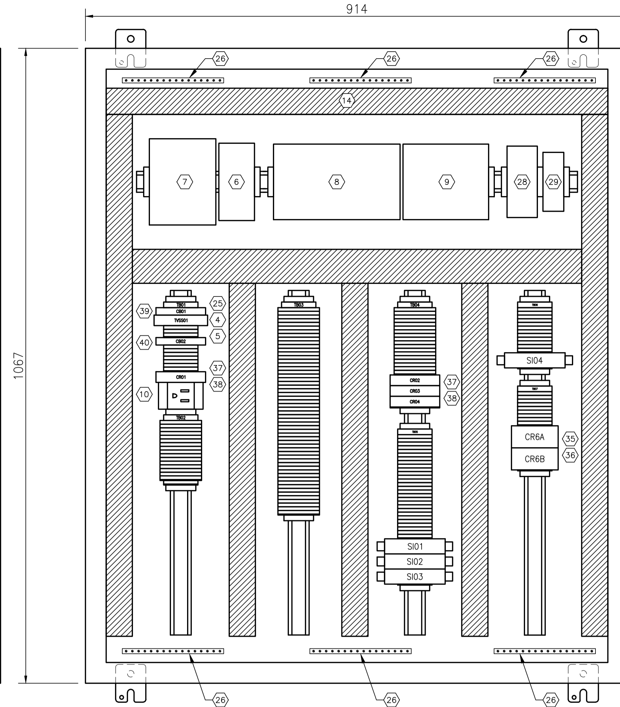
INTERIOR PANEL VIEW SCALE: 1:4
