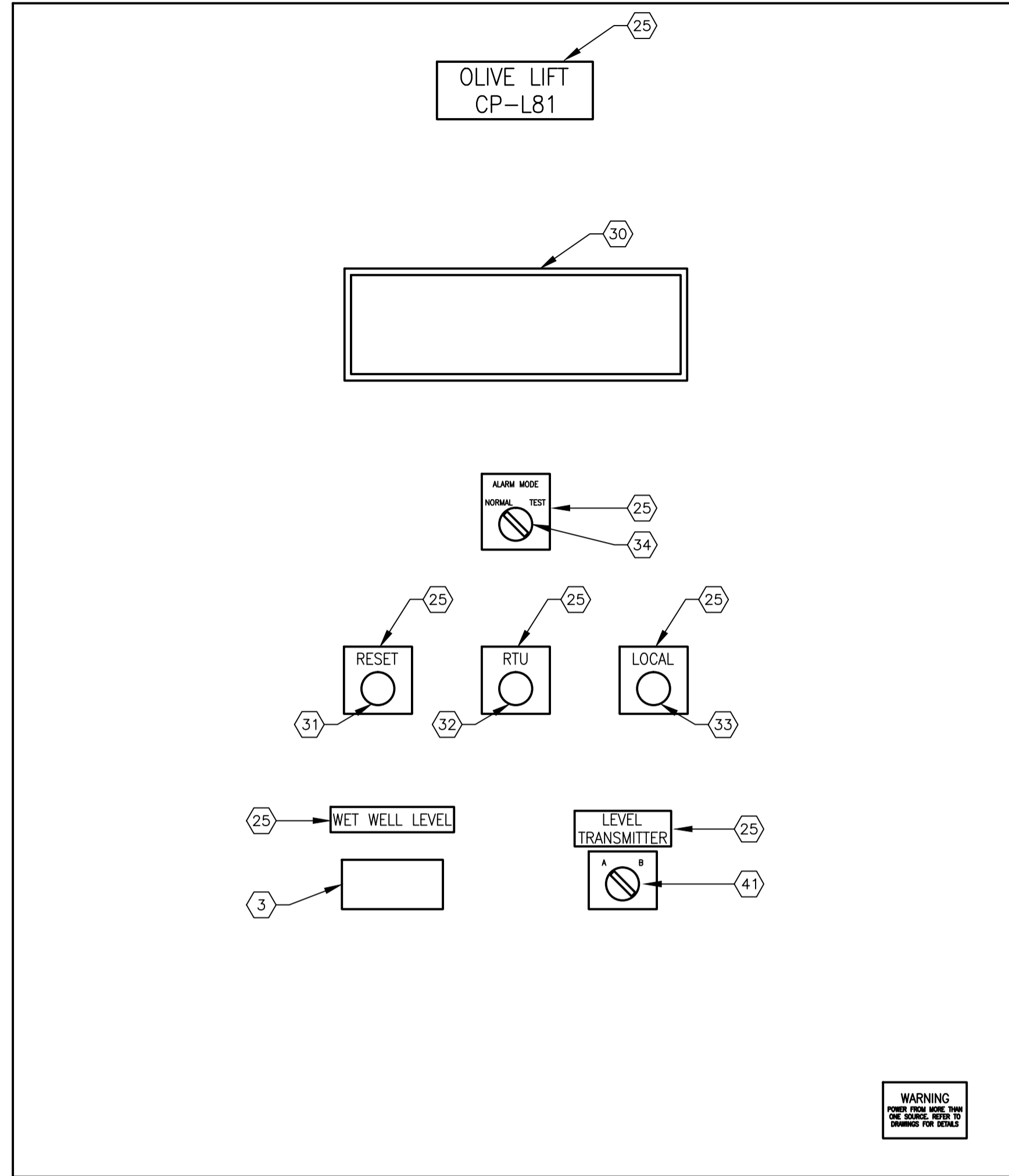
EXTERIOR PANEL VIEW SCALE: 1:4
