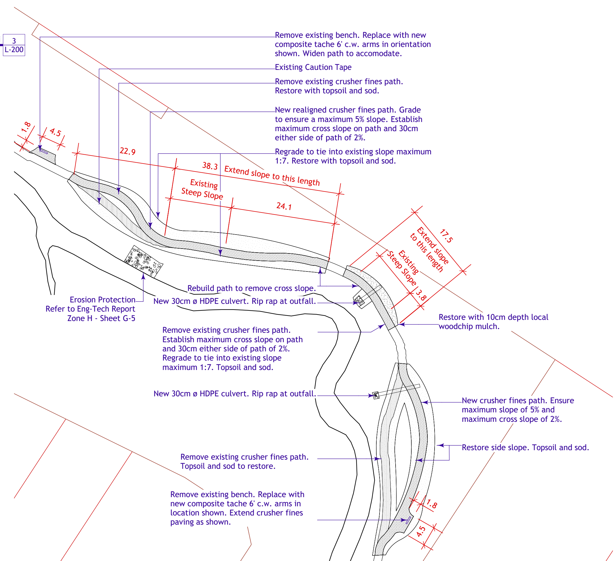
3 Path Rehabilitation Zone ii Scale: 1:500
