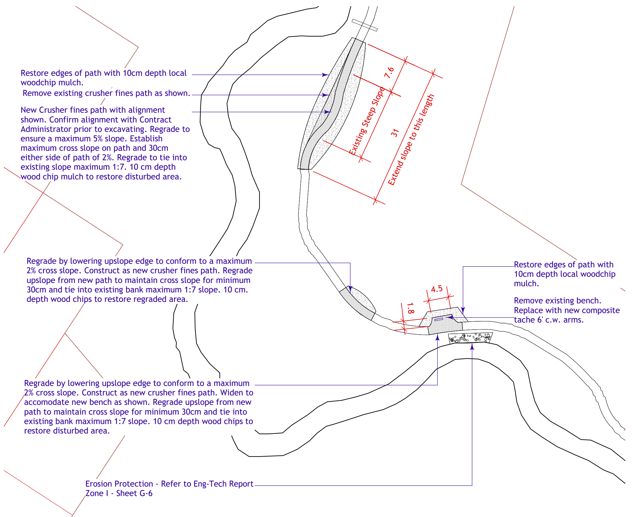
2 Path Rehabilitation Zone i Scale: 1:500
