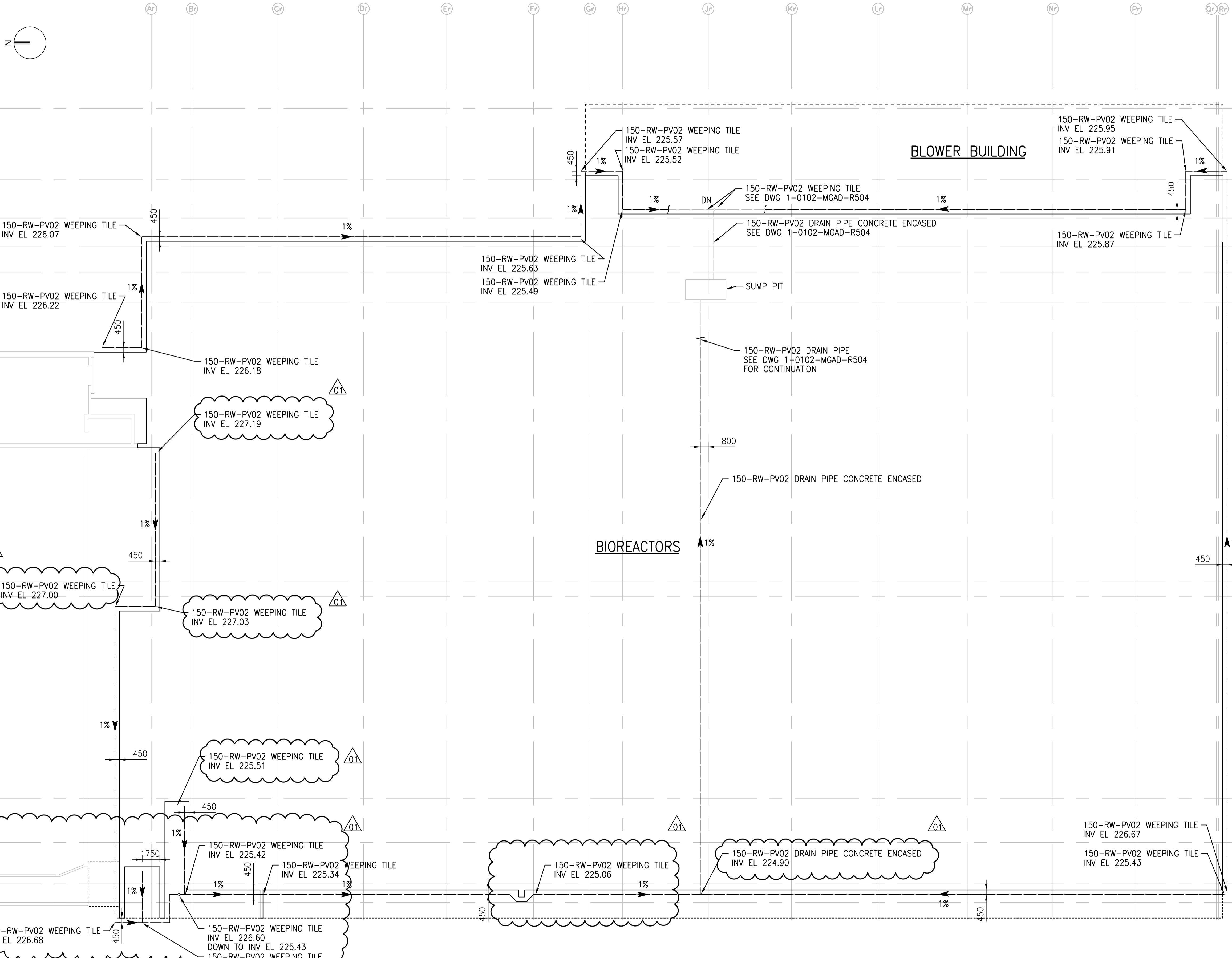
BIOREACTORS/BLOWER BUILDING WEeping TILE PLAN 1:200
