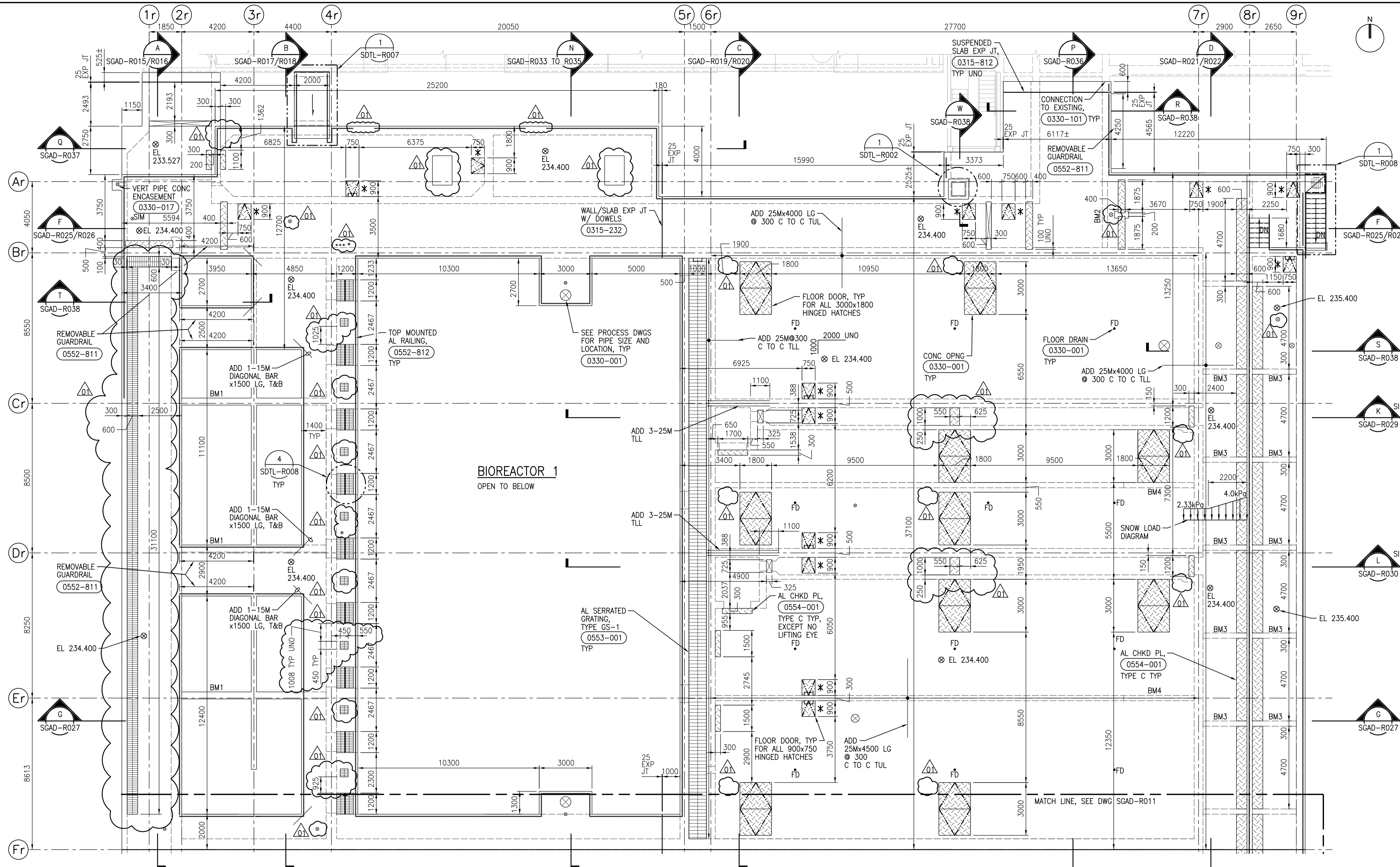
ROOF PLAN 1:100
