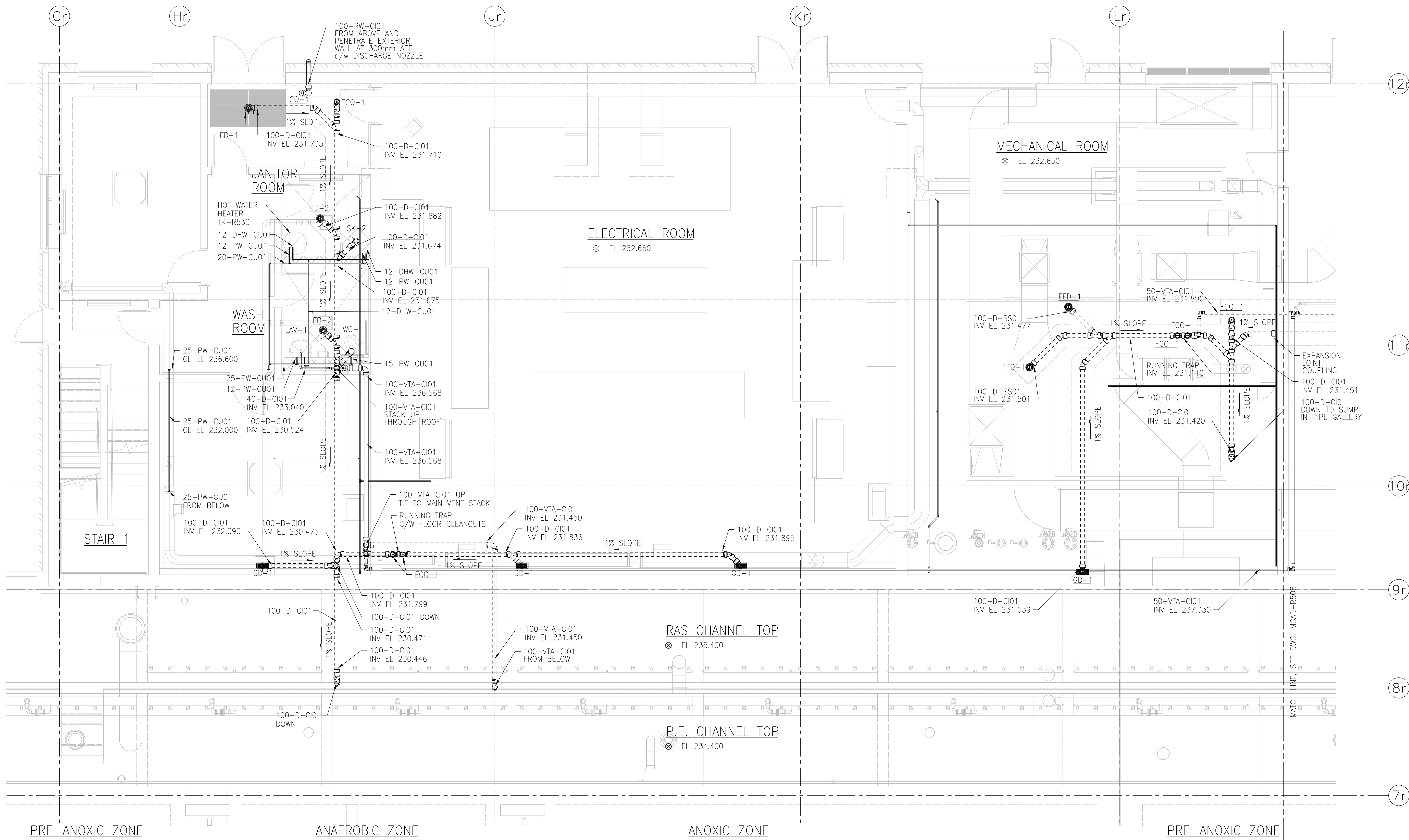
GROUND FLOOR PLAN - PART A 1:50
