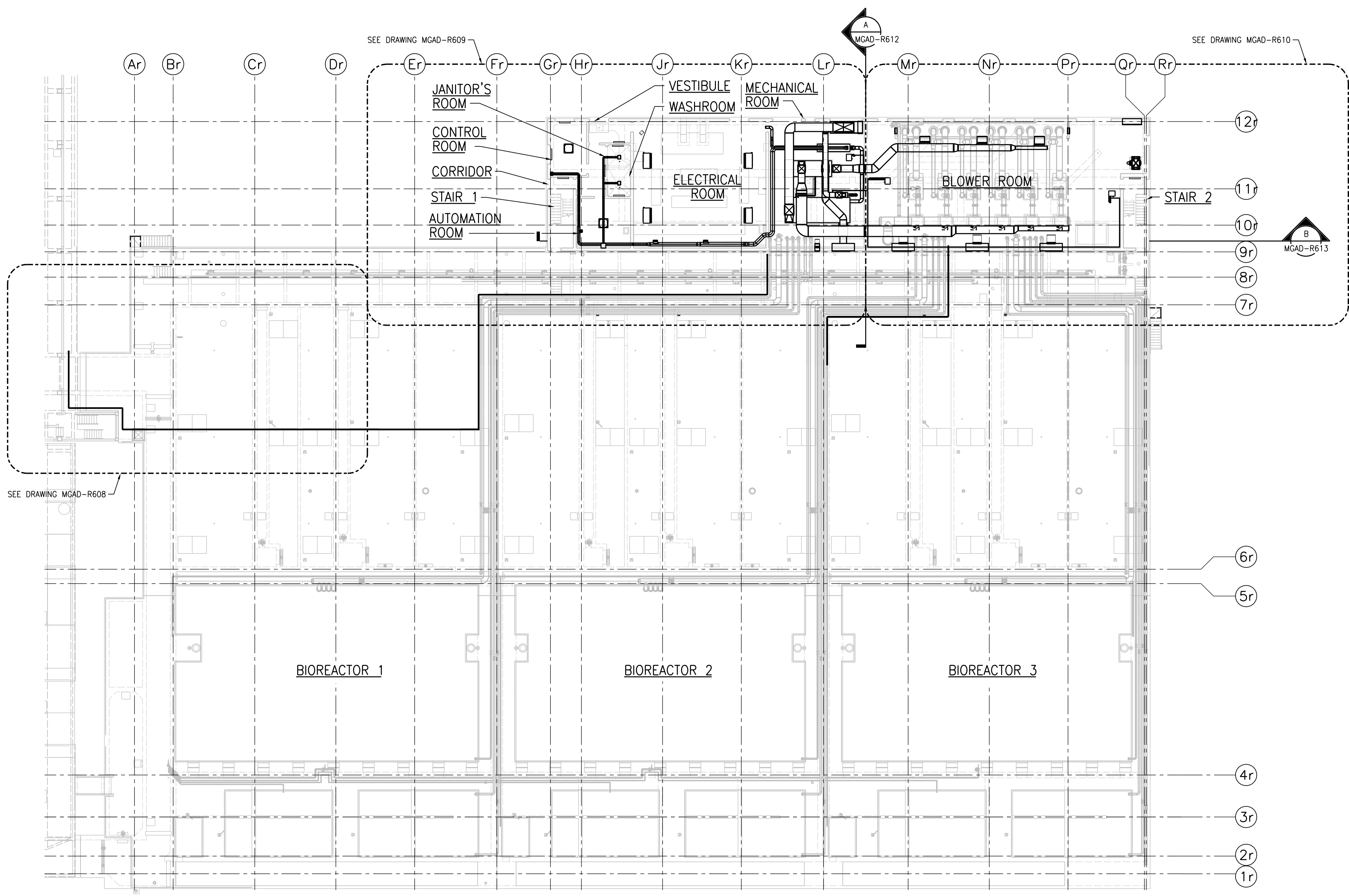
OVERALL GROUND FLOOR PLAN 1:200
