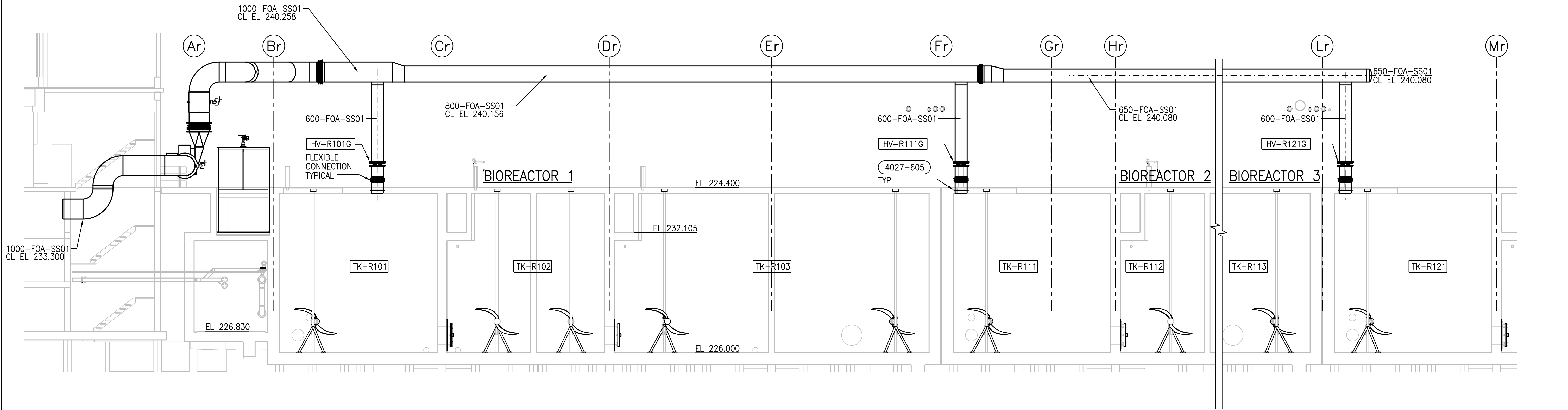
B SECTION 1:100 MGAD-R621
