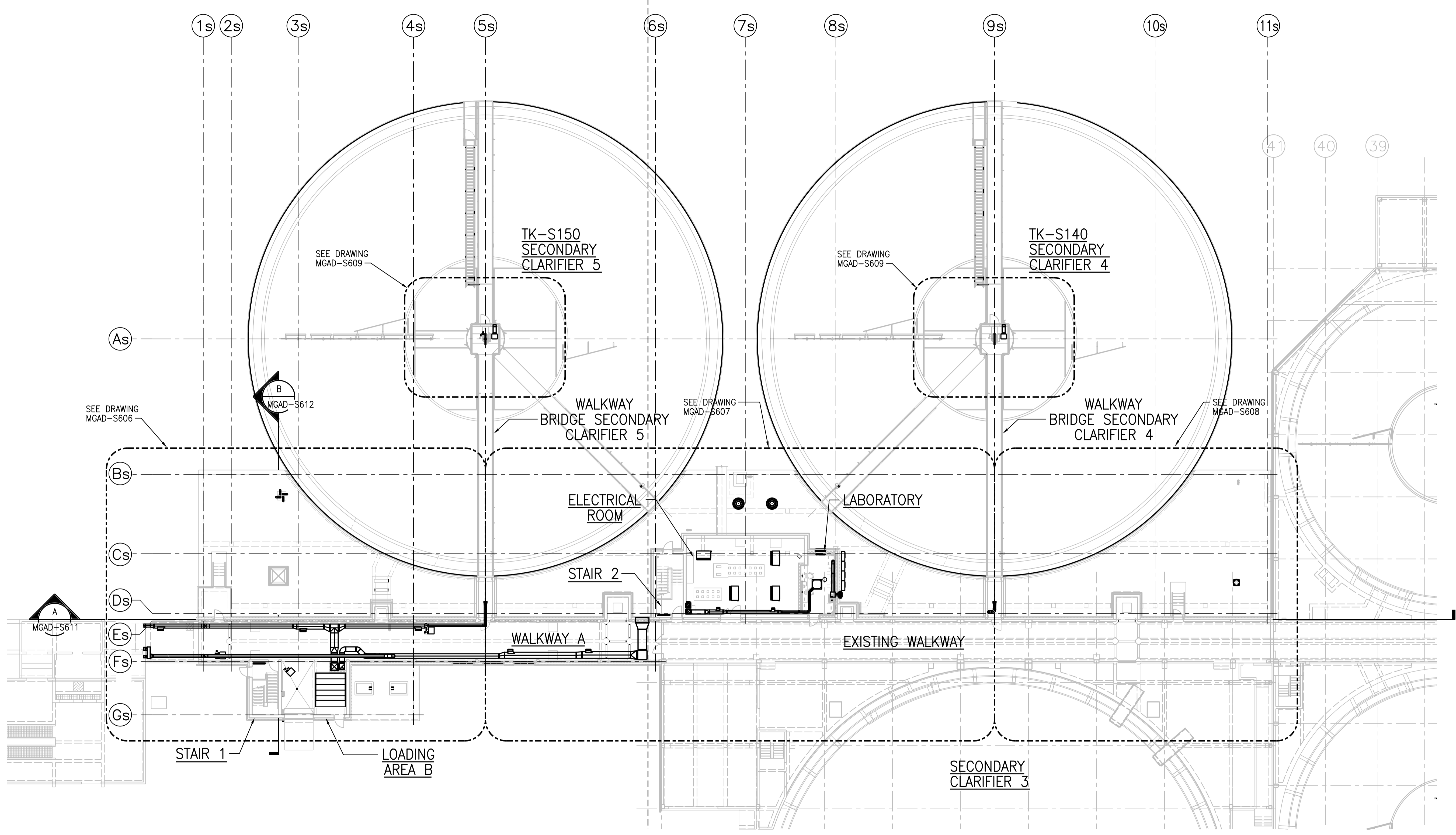
OVERALL GROUND FLOOR PLAN 1:200
