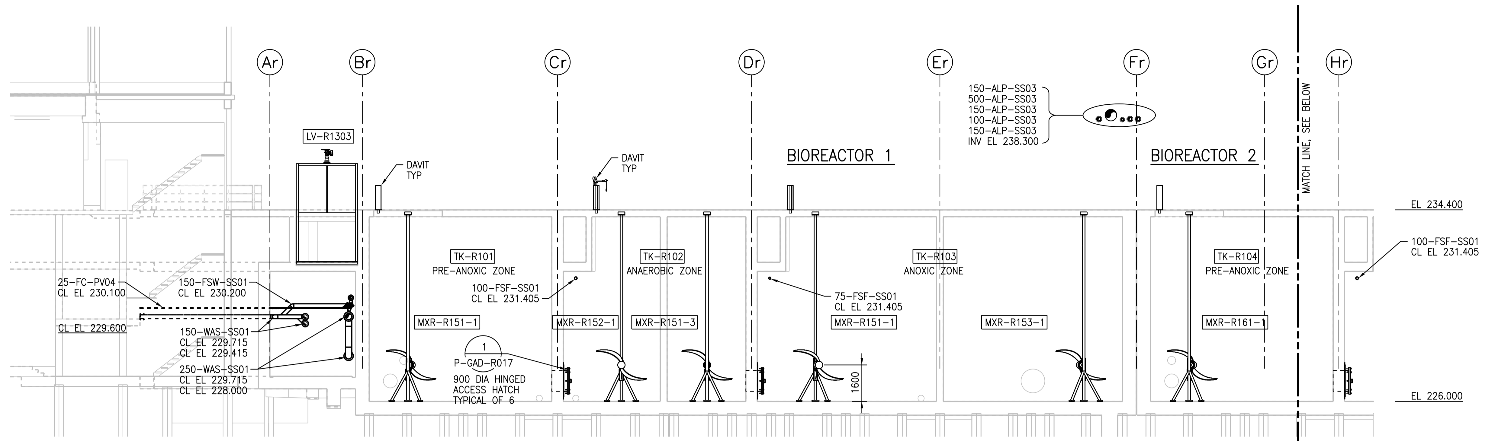
K SECTION - PART A 1:100 PGAD-R001 PGAD-R005 PGAD-R009
