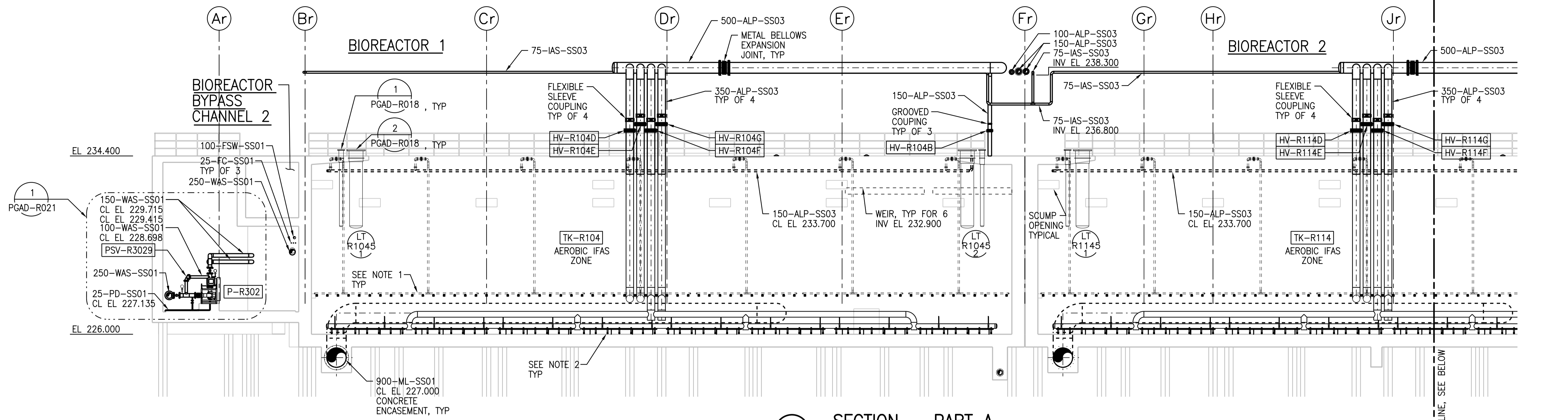
L SECTION - PART A 1:100 PGAD-R001 PGAD-R005 PGAD-R009
