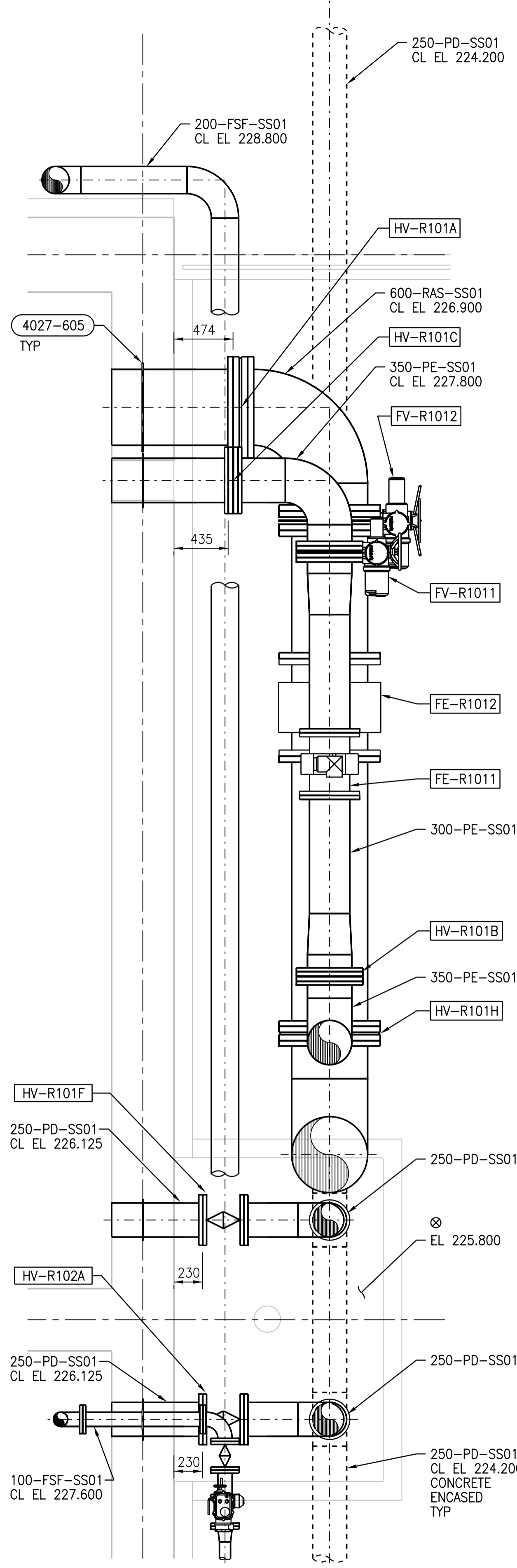
1 DETAIL 1:25
