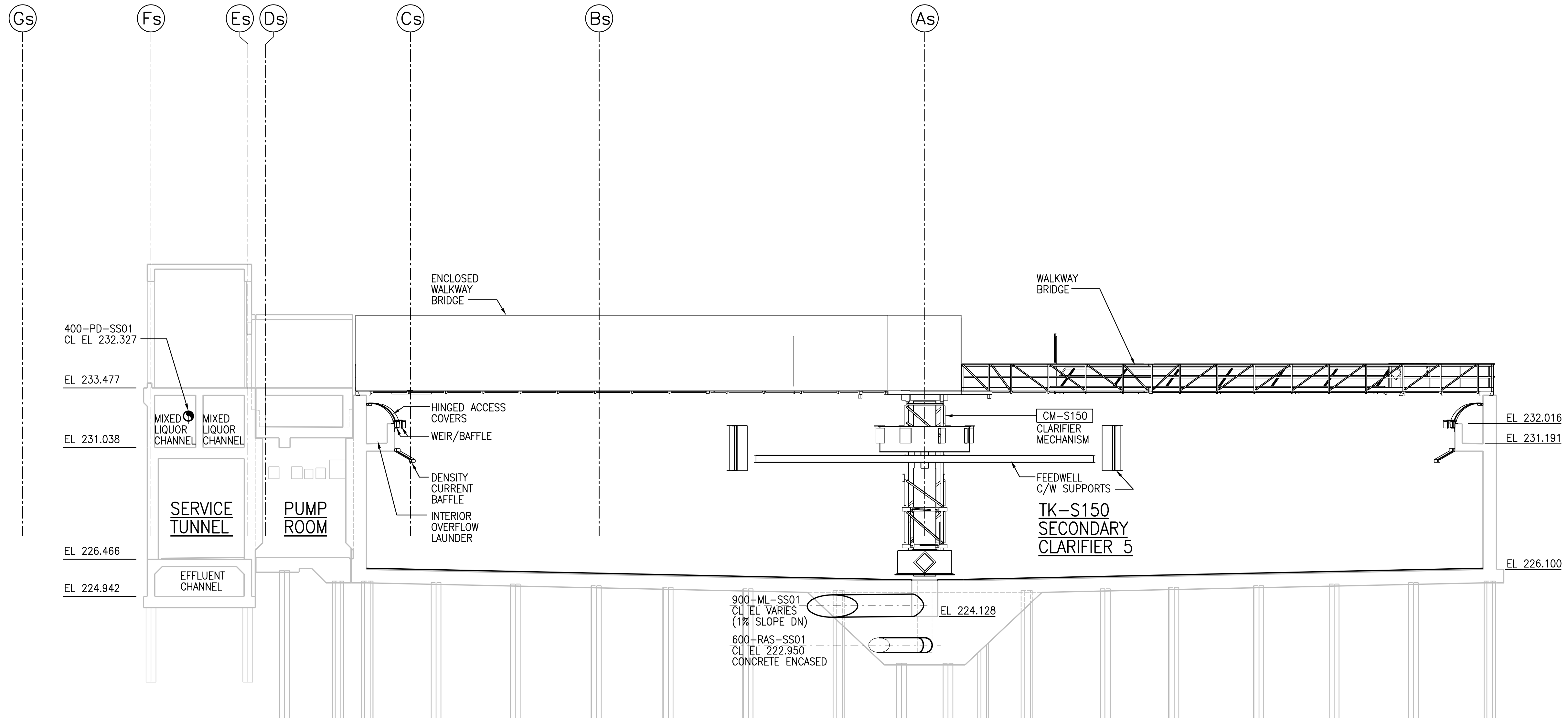
A SECTION 1:100 PGAD-S001 PGAD-S002 PGAD-S003
