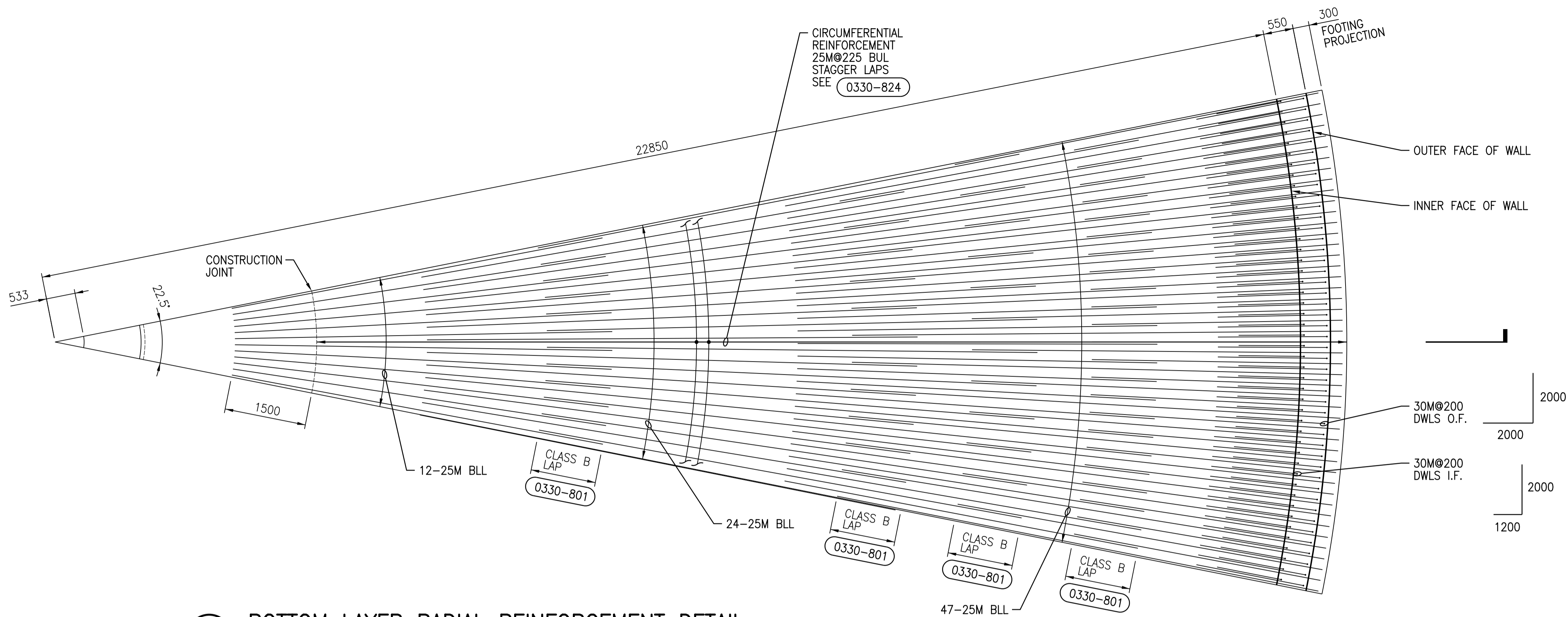
1 BOTTOM LAYER RADIAL REINFORCEMENT DETAIL 1:50 SGAD-S003
