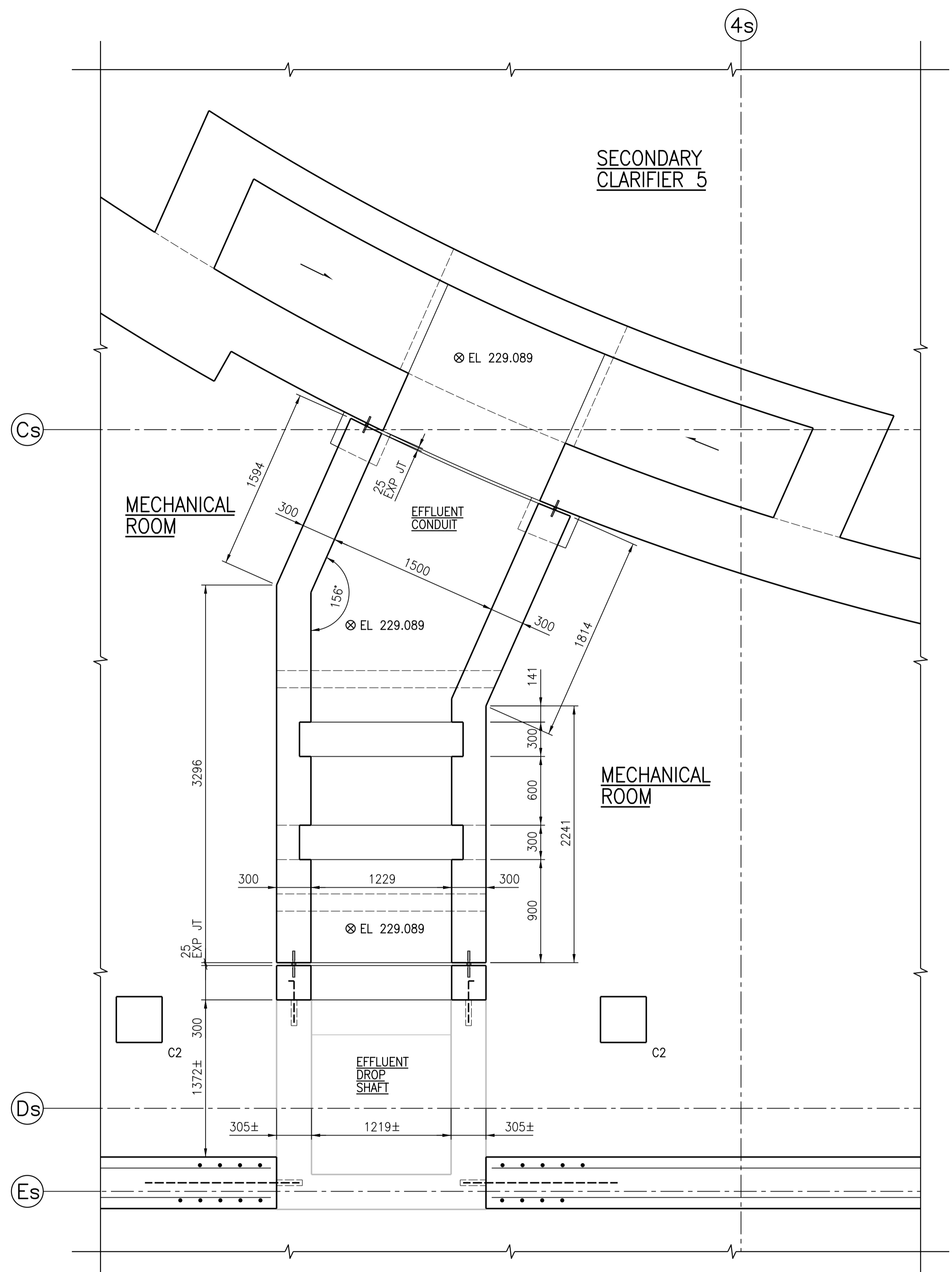
1 DETAIL 1:25 SGAD-S009
