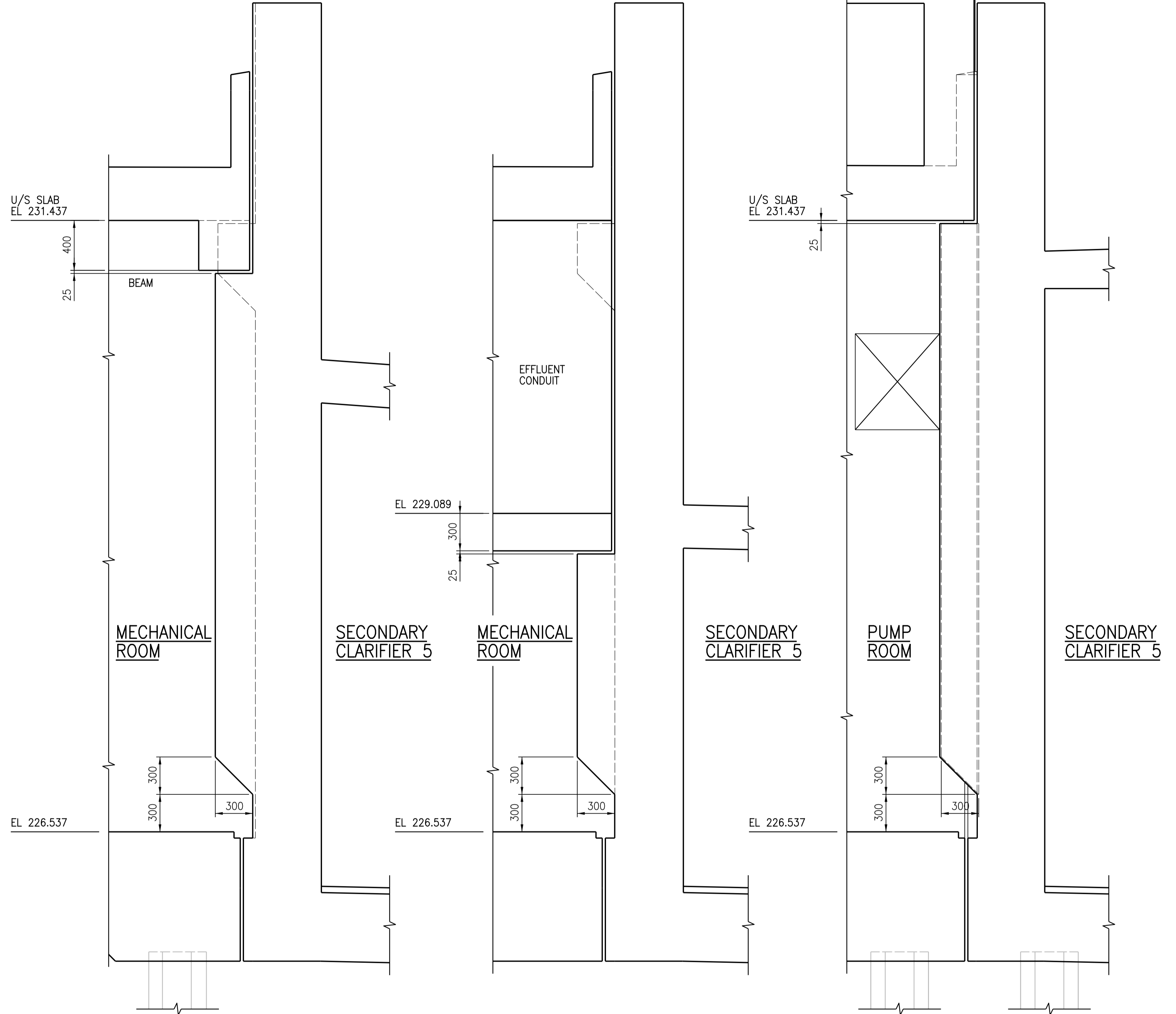
3 DETAIL 1:20 SDTL-S005
