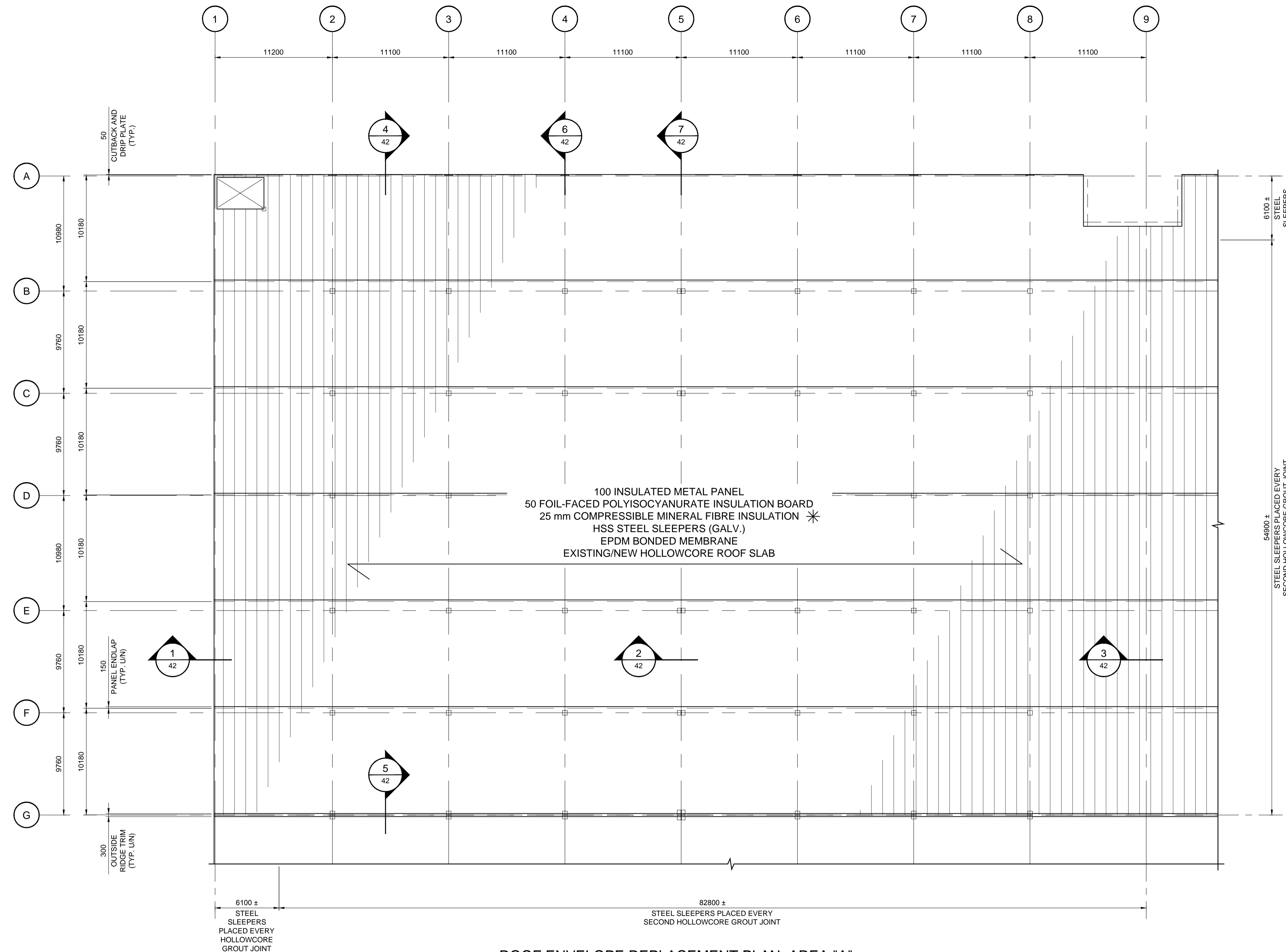
ROOF ENVELOPE REPLACEMENT PLAN, AREA "A" 1:200
