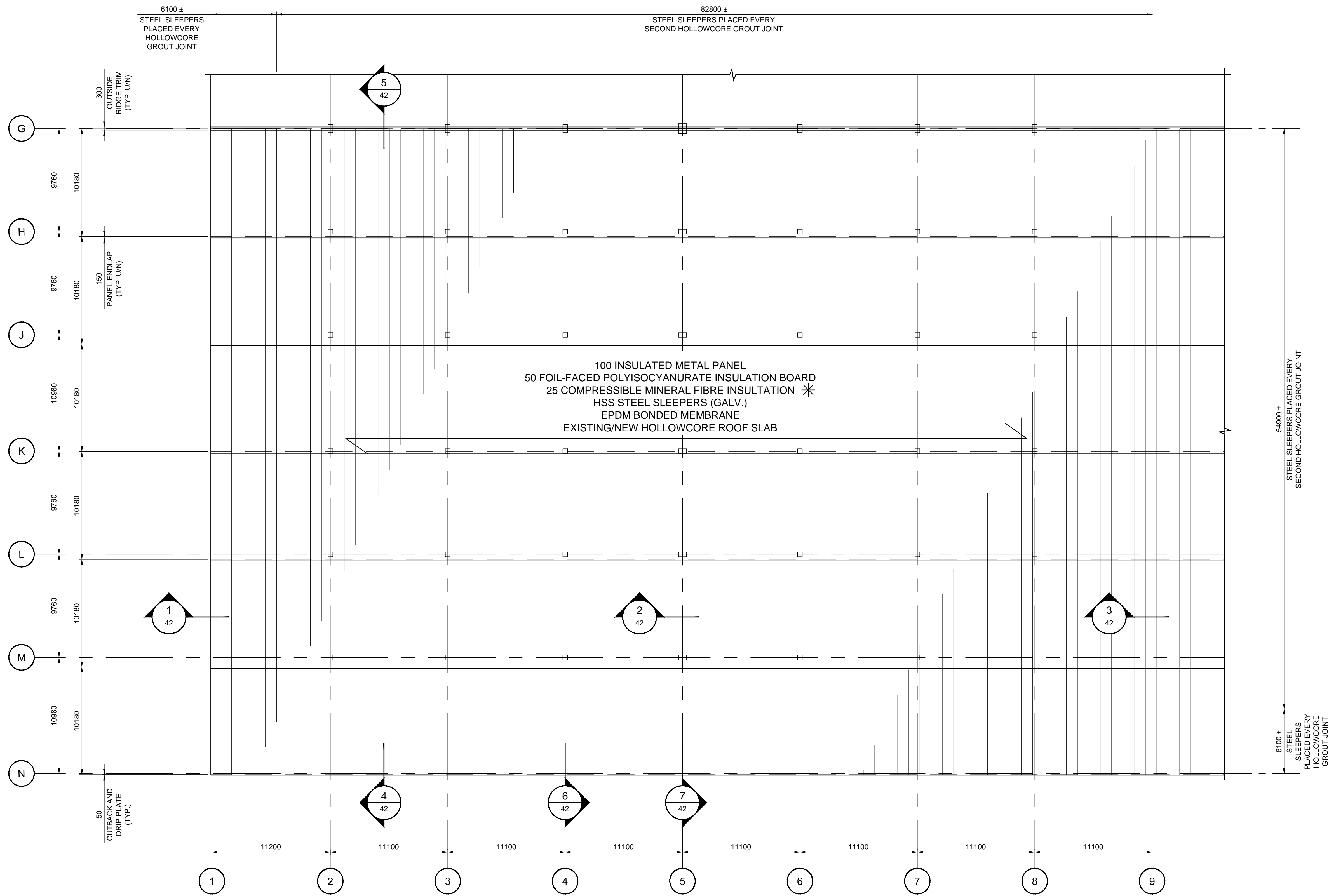
ROOF ENVELOPE REPLACEMENT PLAN, AREA "C" 1:200
