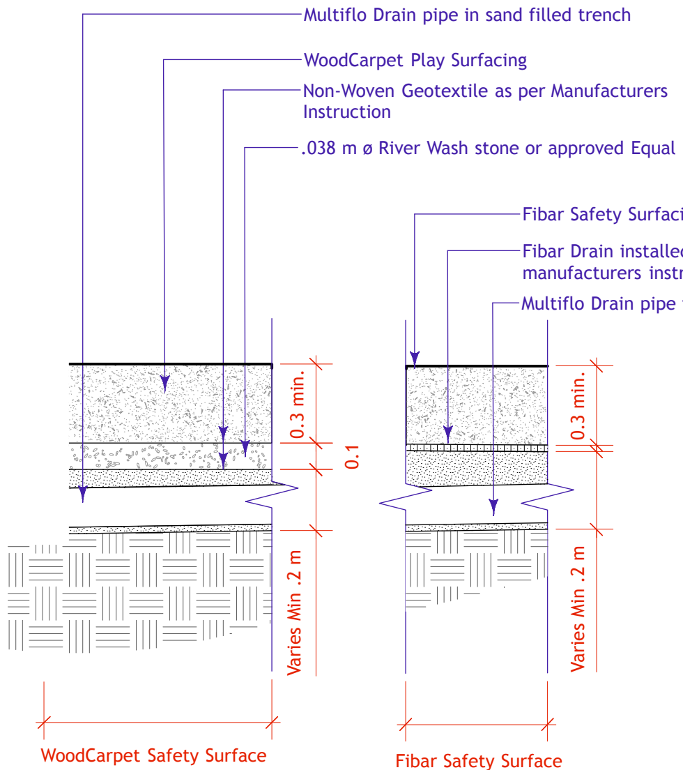
2 Playground Safety Surfacing and Subdrain L-2 Scale: 1:20
