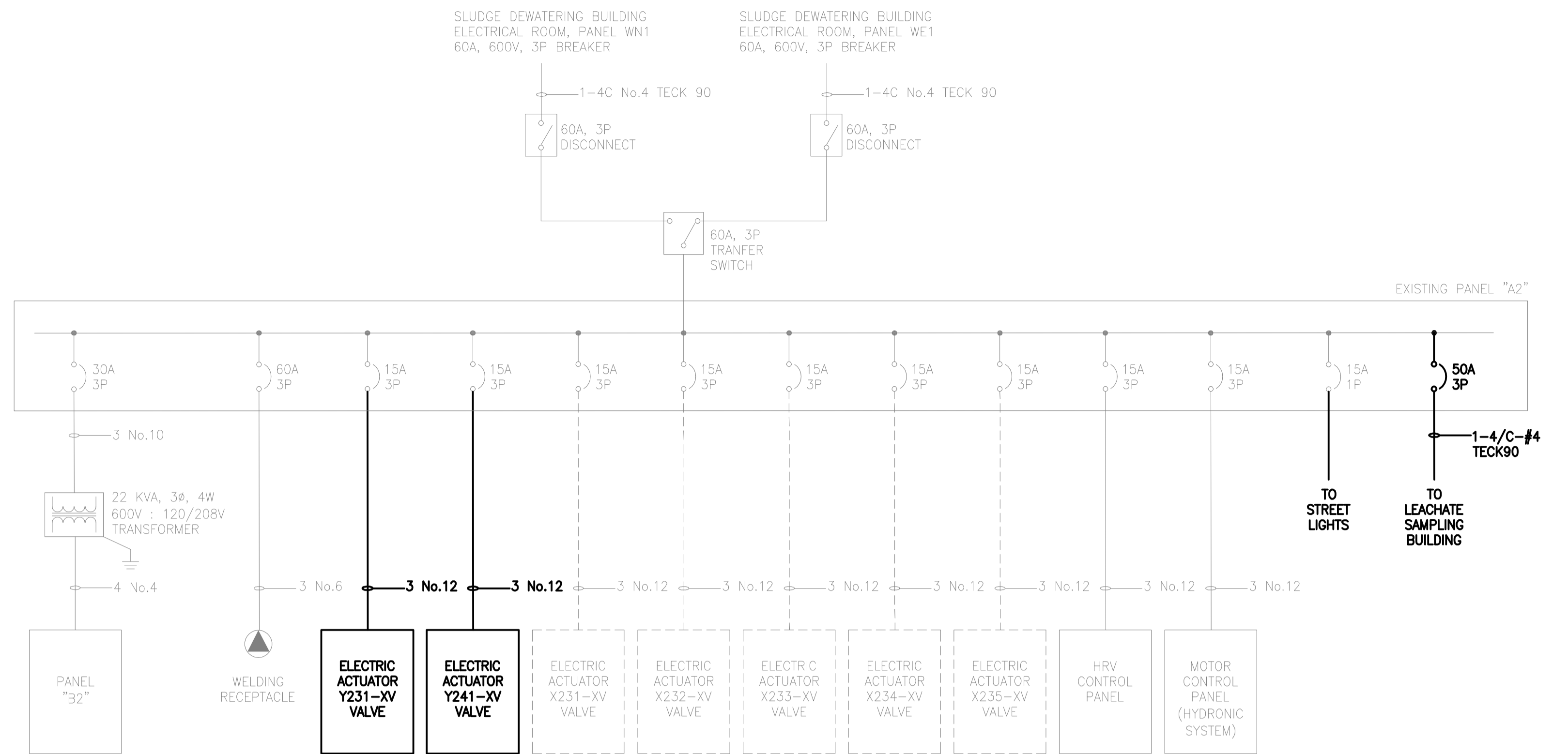
2 HAULED WASTEWATER BUILDING NO. 2 - SINGLE LINE DIAGRAM E0013 N.T.S. (FORMERLY LEACHATE RECEIVING BUILDING)
