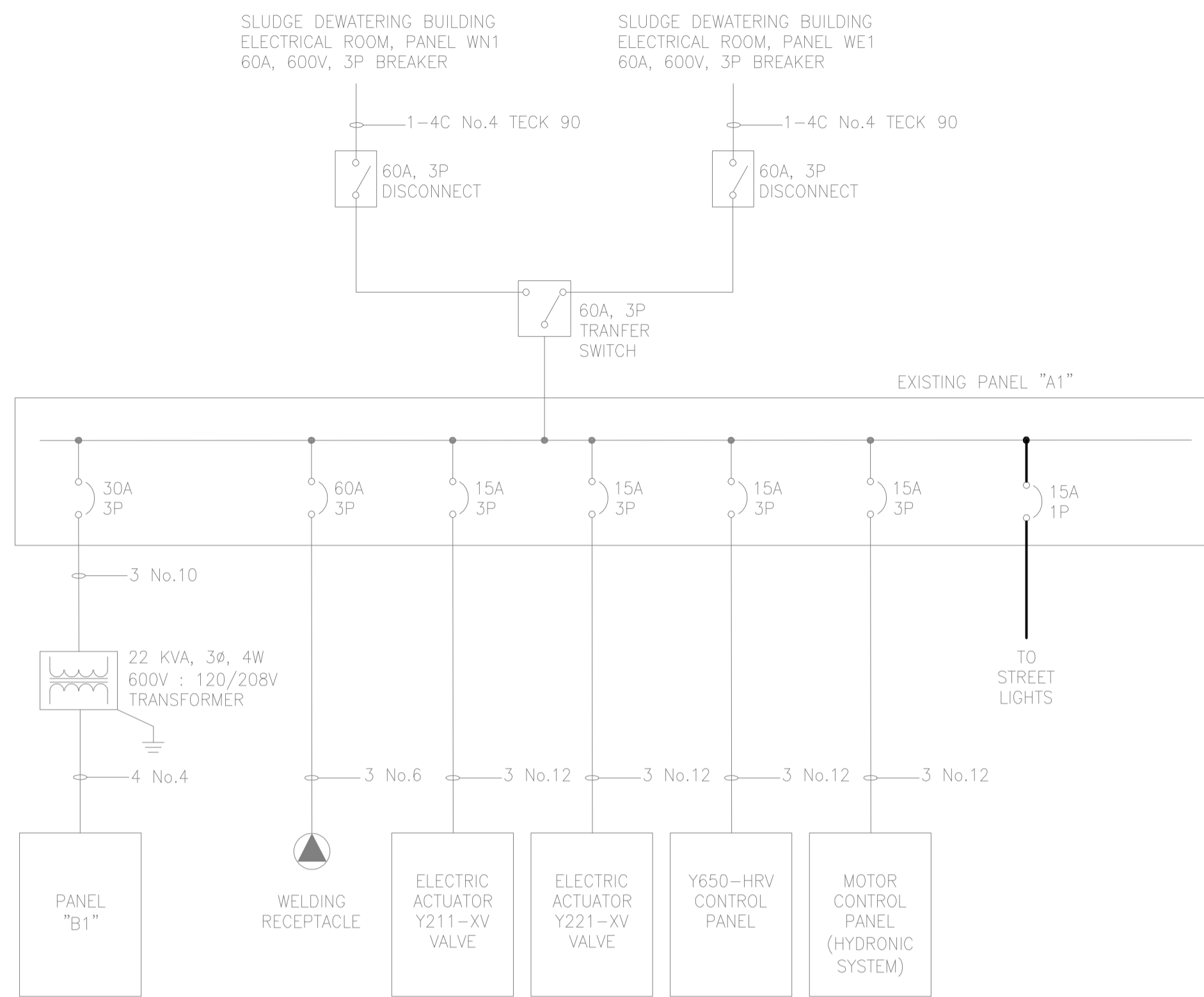
1 HAULED WASTEWATER BUILDING NO. 1 - SINGLE LINE DIAGRAM E0013 N.T.S. (FORMERLY HAULED WASTEWATER BUILDING)
