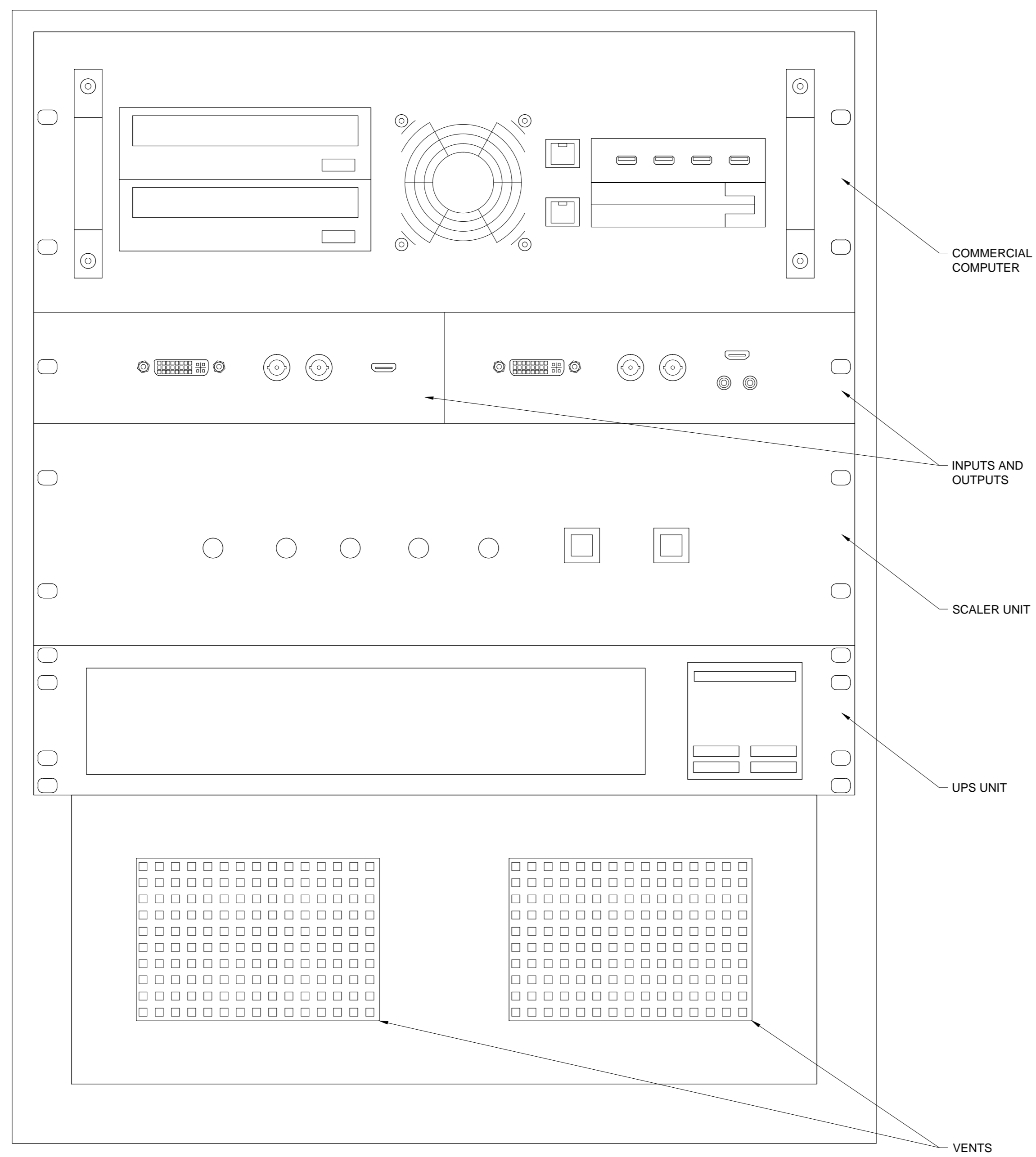
TYPICAL VIDEO RACK DETAIL 2 NOT TO SCALE AQ104
