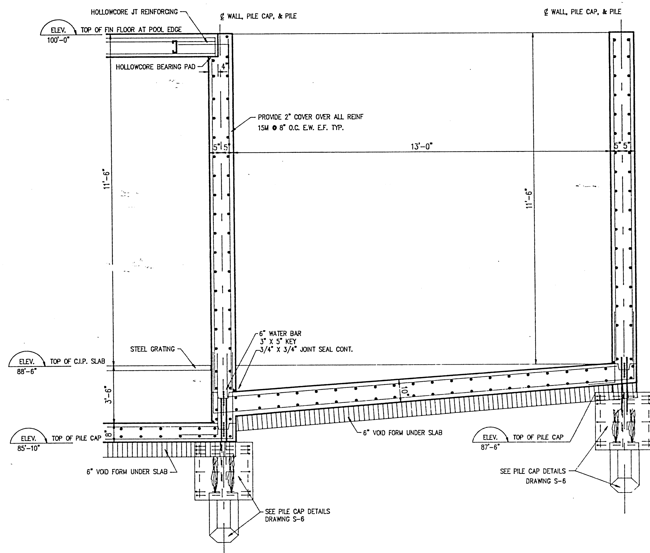
1 SURGE TANK 12 SCALE 1/2" = 1'-0"
